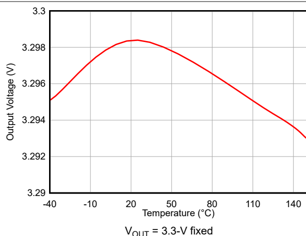
図 6-3. Output Voltage Accuracy Versus Temperature
