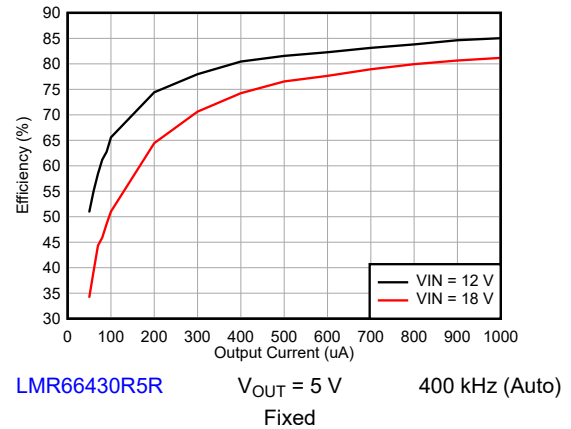
図 8-5. Efficiency
