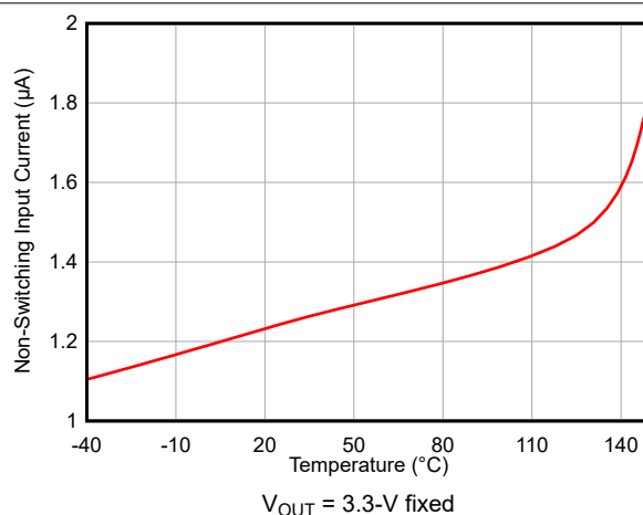
図 6-2. Non-Switching Input Current ( I_{QVIN(nonsw)} ) Versus Temperature
