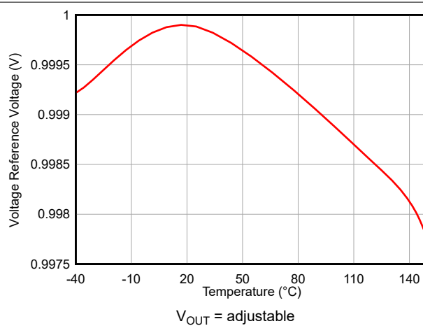
図 6-4. Feedback Voltage Accuracy Versus Temperature
