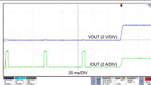
Figure 7-15. Hiccup Exit
