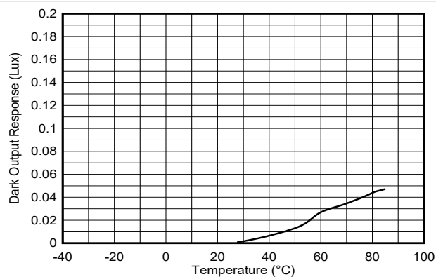
FIG 7-3. Dark Response vs Temperature
