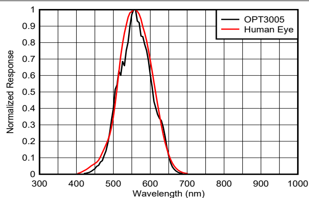
FIG 7-2. Spectral Response vs Wavelength
