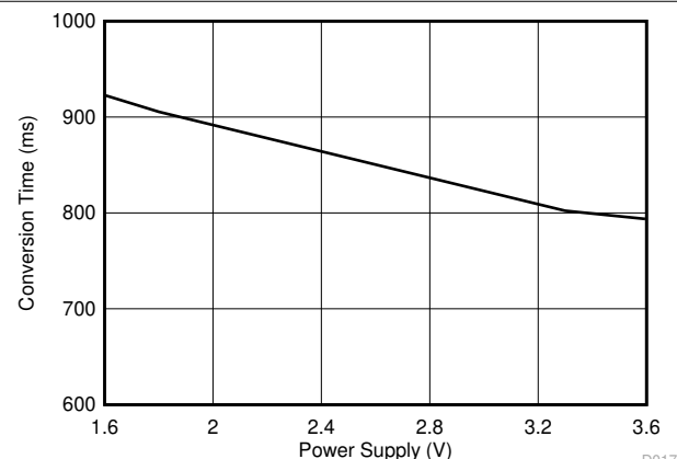
FIG 7-5. Conversion Time vs Power Supply
