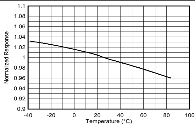
FIG 7-4. Normalized Response vs Temperature
