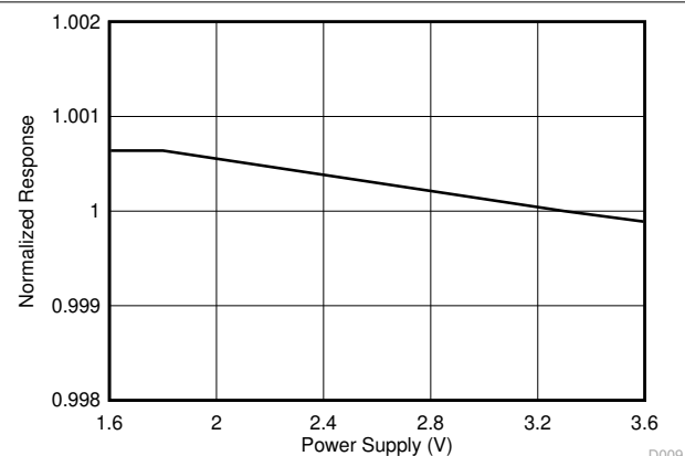
FIG 7-6. Normalized Response vs Power-Supply Voltage
