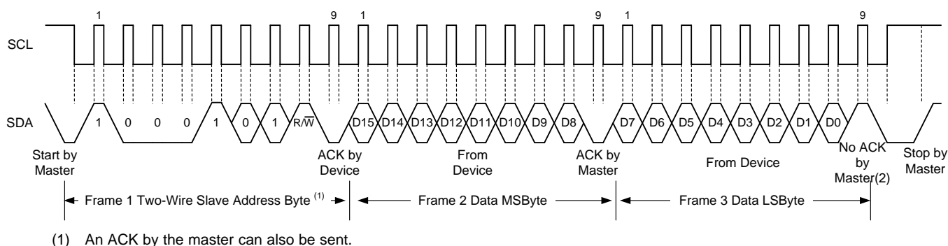
Figure 21. I 2 C Read Example
