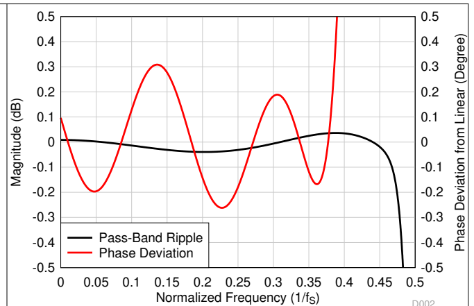
図 7-42. Low-Latency Decimation Filter Pass-Band Ripple and Phase Deviation
