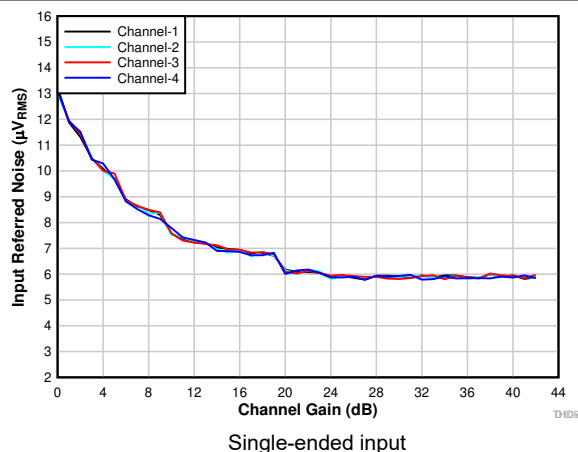
図 6-11. Input-Referred Noise vs Channel Gain
