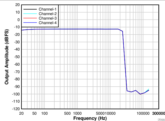
図 6-12. Frequency Response With a -12-dBr Input
