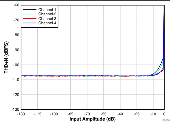
8-3. THD+N vs Input Amplitude
