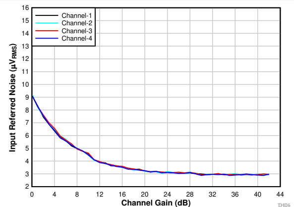
Figure 6-10. Input-Referred Noise vs Channel Gain
