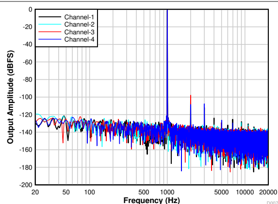
図 6-16. FFT With a -1-dBr Input
