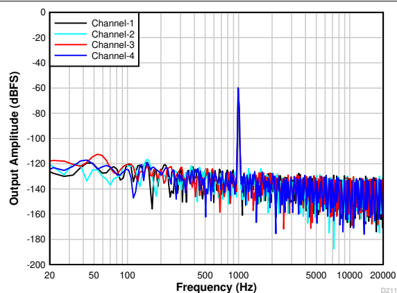
8-2. FFT With a -60-dBr Input
