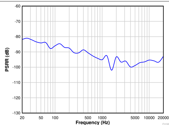
図 6-13. Power-Supply Rejection Ratio vs Ripple Frequency With 100-mV PP Amplitude
