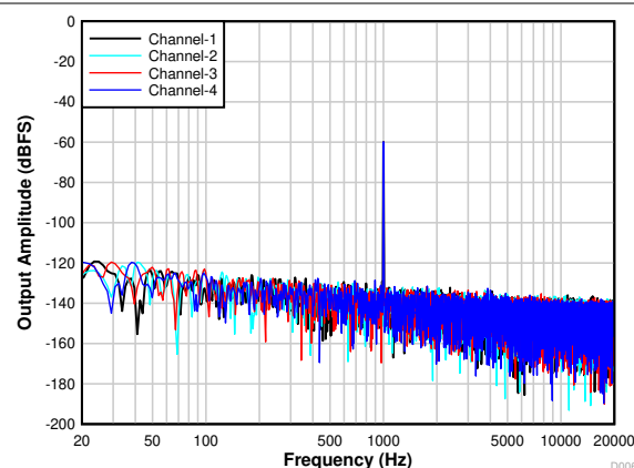
図 6-15. FFT With a -60-dBr Input
