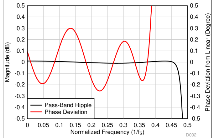
図 7-40. Low-Latency Decimation Filter Pass-Band Ripple and Phase Deviation
