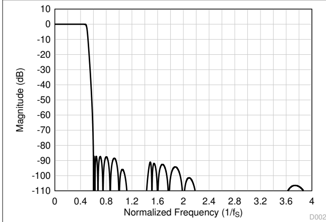
図 7-39. Low-Latency Decimation Filter Magnitude Response
