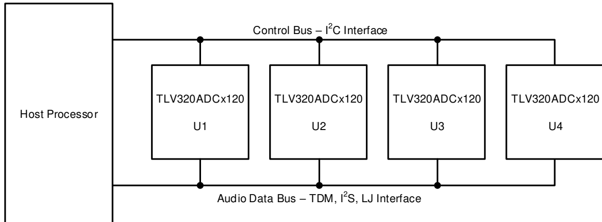
図 7-13. Multiple PCM3140-Q1 Devices With Shared Control and Audio Data Buses
