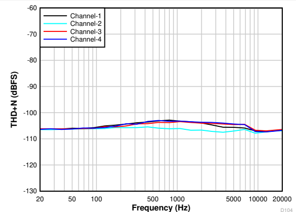
Figure 6-9. THD+N vs Input Frequency With a -1\text{-dBr} Input
