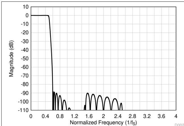
図 7-41. Low-Latency Decimation Filter Magnitude Response
