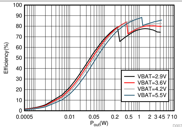
FIG 13. Efficiency vs Output Power
