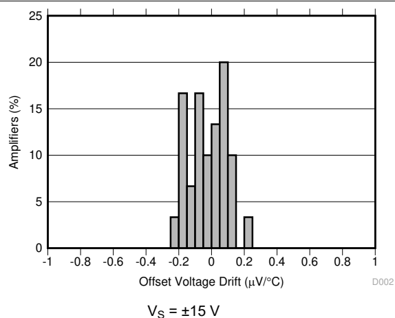
Figure 6-3. Input Offset Voltage Drift Histogram
