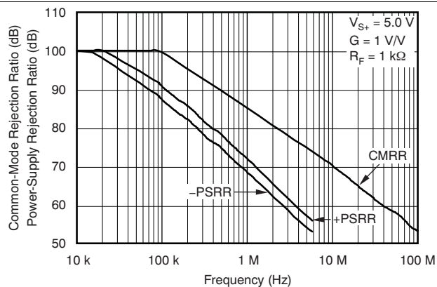
Figure 44. Rejection Ratio vs Frequency
