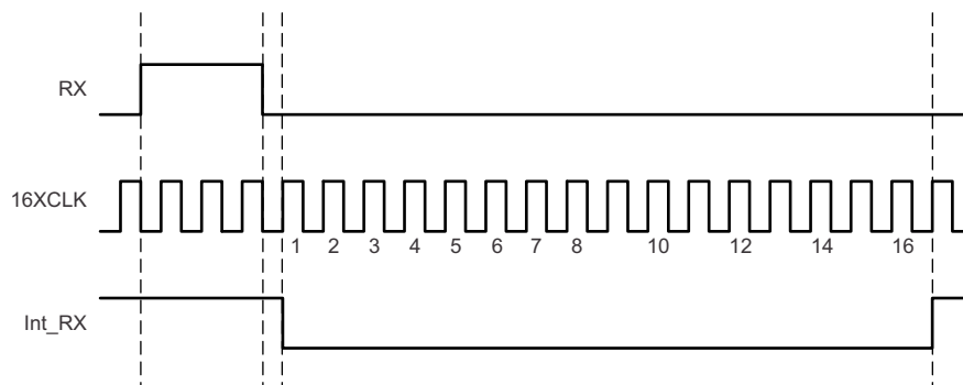
FIG 41. Positive RX Pulse Decode – Detailed View
