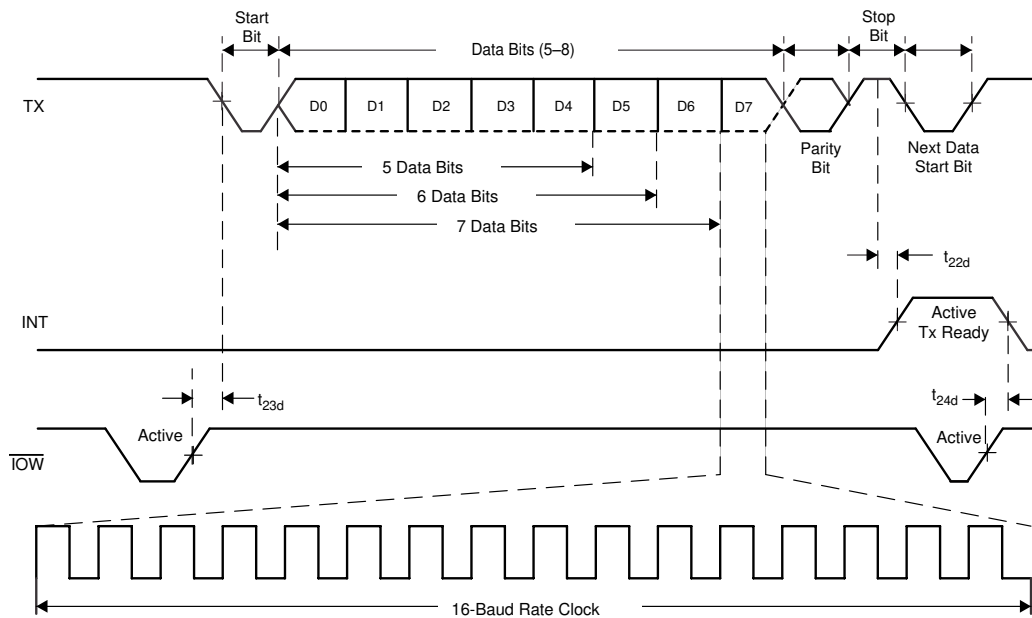
✕ 14. Transmit Timing ( \overline{\text{IOR}} and \overline{\text{IOW}} Mode, \text{MODE} = \text{VCC} )
