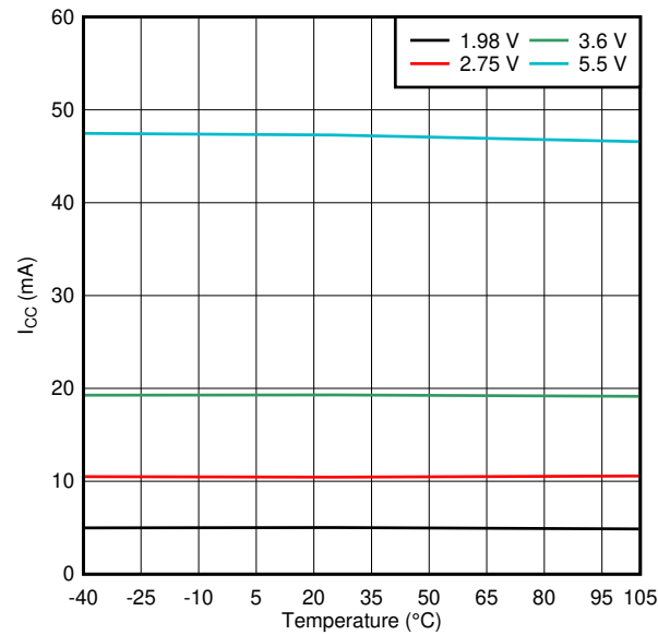
FIG 1. I CC vs Temperature
