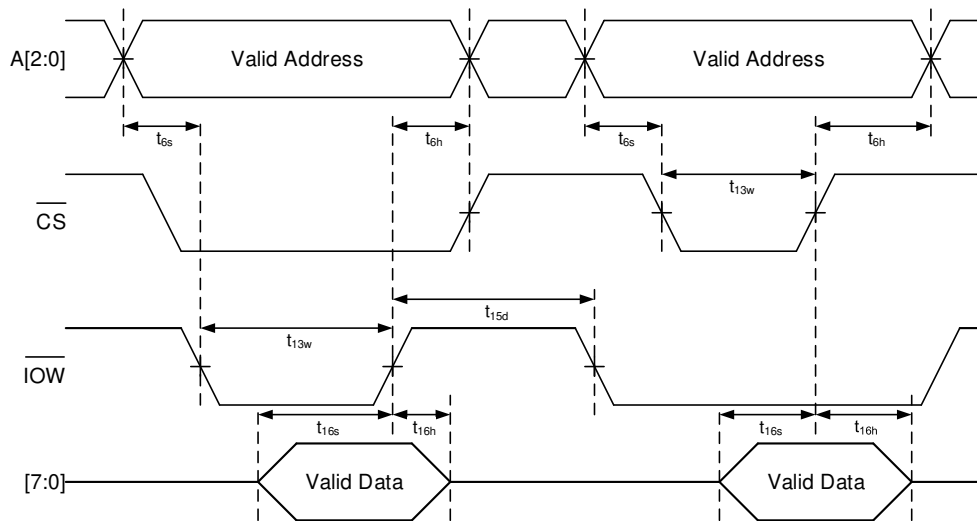
FIG 2. General Write Timing ( \overline{\text{I/O}} and \overline{\text{IOW}} Mode, MODE = VCC)
