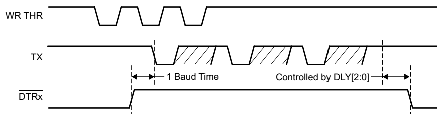
图 31. \overline{\text{DTRx}} and Transmit Data Relationship
