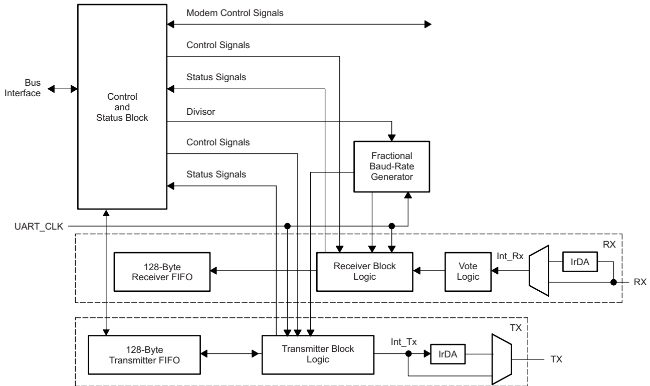
FIG 19. TL16C750E Functional Block Diagram – Control Blocks
