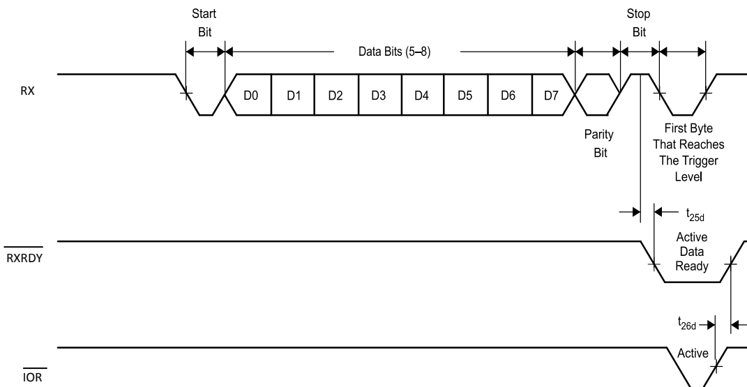
✎ 12. Receive Timing in FIFO Mode ( \overline{\text{IOR}} and \overline{\text{IOW}} Mode, MODE = VCC)
