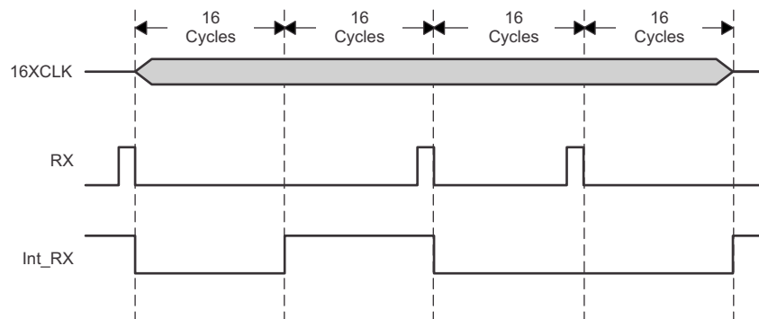
FIG 42. Positive RX Pulse Decode – Macro View
