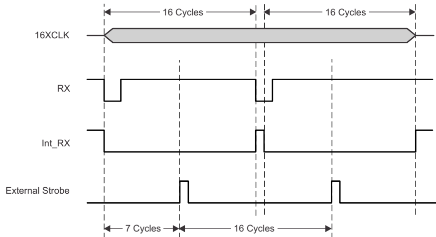
FIG 40. Recommended Strobing for Decoded Data
