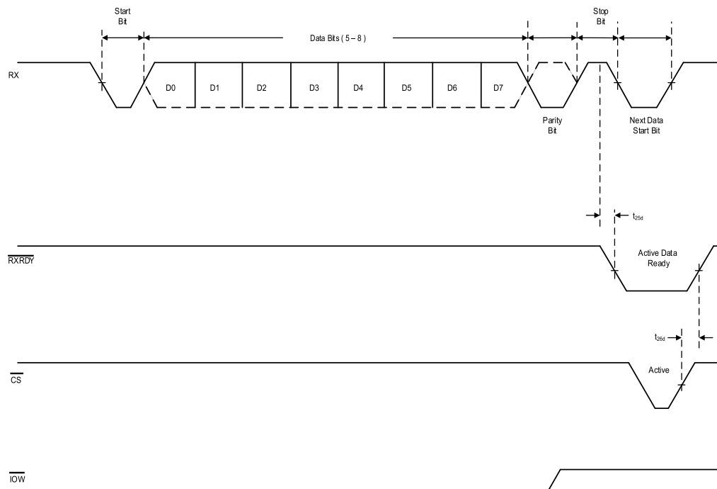
✎ 11. Receive Ready Timing in Non-FIFO Mode ( \overline{\text{IOW}} Only Mode, MODE = GND)
