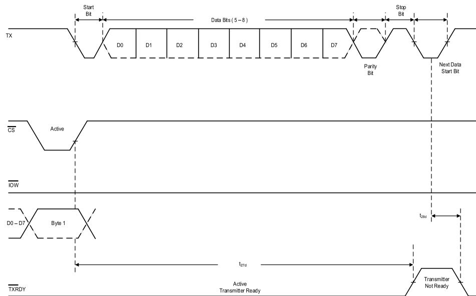
FIG 17. Transmit Ready Timing in Non-FIFO Mode ( \overline{IOW} Only Mode, MODE = GND)
