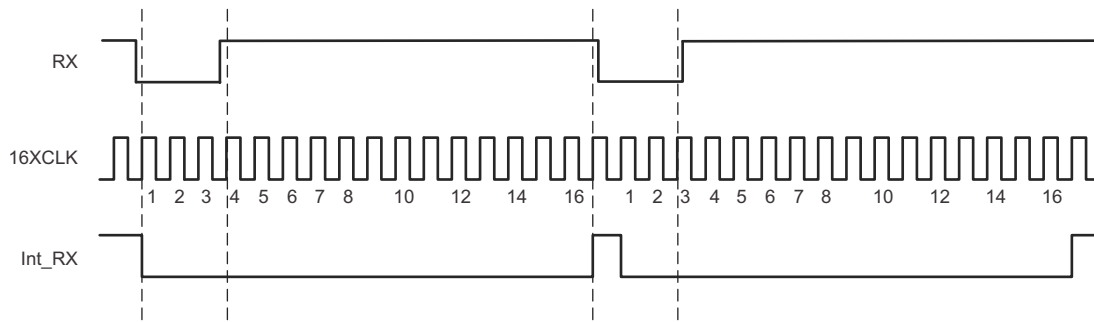
FIG 39. Timing Causing 1-Clock-Wide Pulse Between Consecutive Ones
