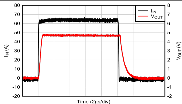
図 6-11. Current Overload Response
