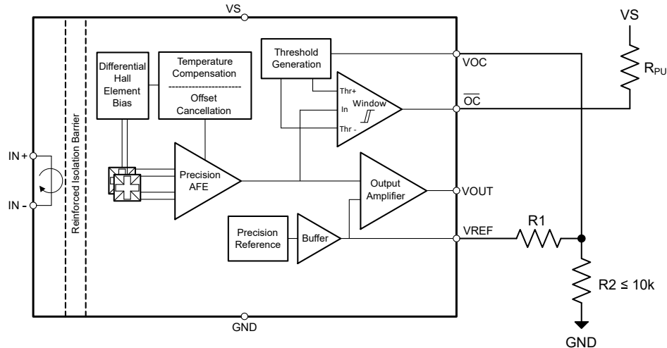
図 8-6. User Configurable Overcurrent Threshold Using Zero Current Output Reference Voltage
