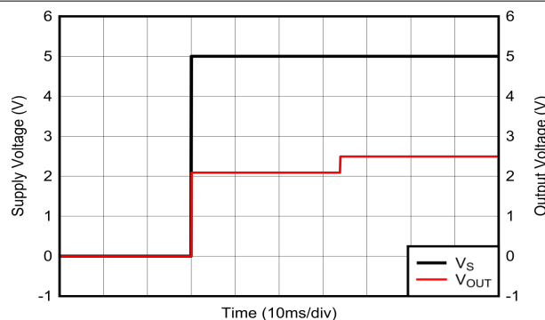
図 6-12. Startup Transient Response
