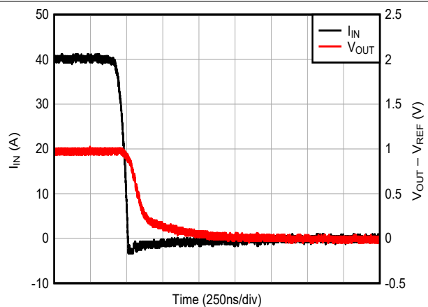
図 6-10. Voltage Output Step Response, Falling
