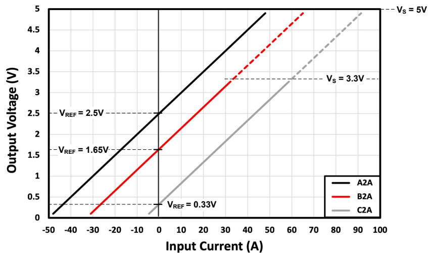
図 8-4. Output Voltage Relationship to Input Current for TMCS1126x2A
