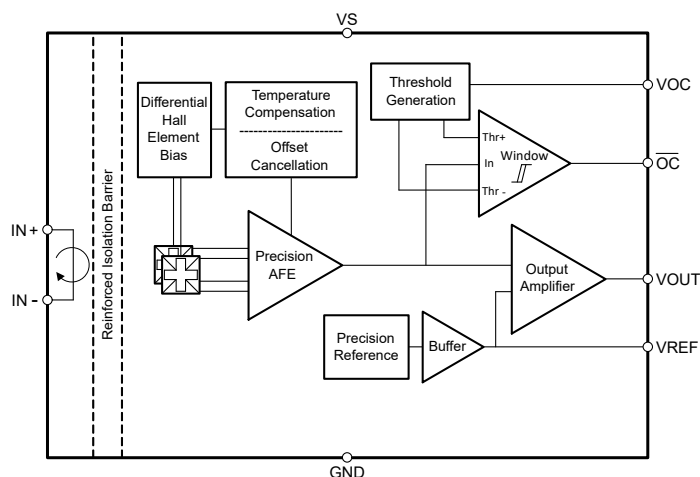
8-1. Function Block Diagram
