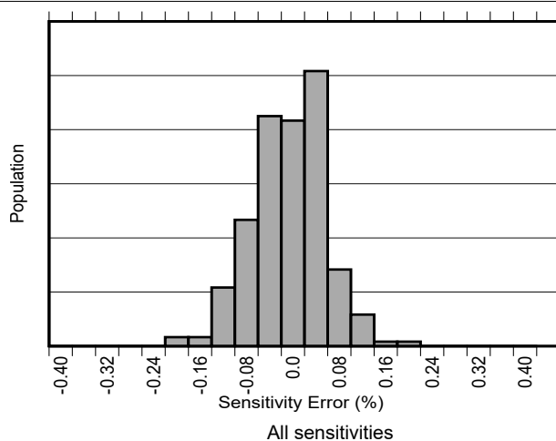
図 6-4. Sensitivity Error Production Distribution: Grade A
