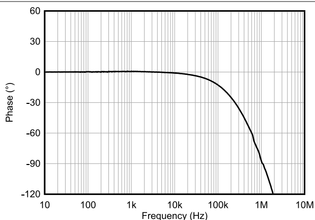
図 6-6. Phase vs Frequency, All Gains
