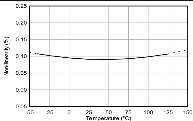
図 6-3. Non-Linearity vs Temperature
