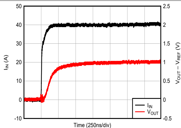
図 6-9. Voltage Output Step Response, Rising
