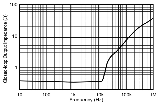
図 6-8. Output Impedance vs Frequency
