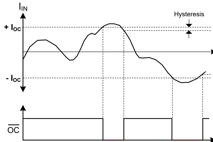
図 8-7. Overcurrent Detection Diagram
