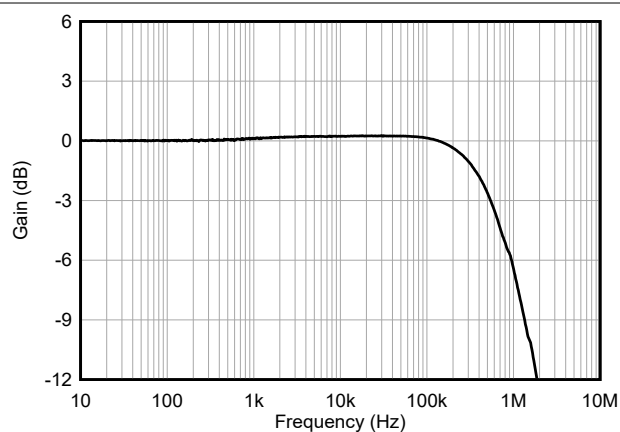
図 6-5. Sensitivity vs Frequency, All Gains Normalized to 1Hz
