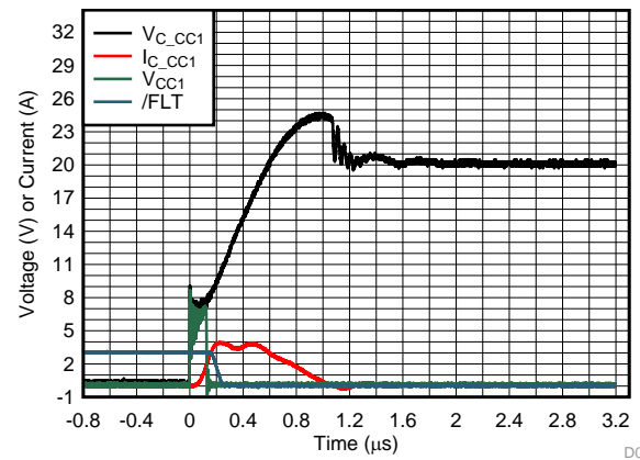
图 2. CC Short-to-VBUS 20-V VM = 3.3 V
