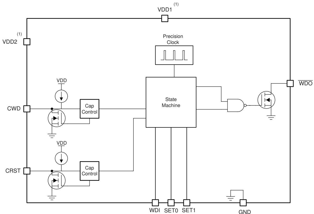
FIG 7-1. TPS3430 Block Diagram
