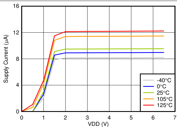
6-5. Supply Current vs Power-Supply Voltage
