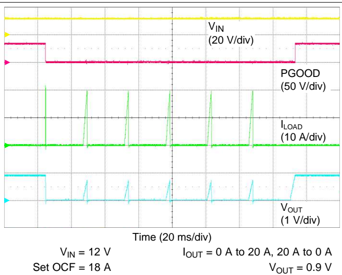
Figure 51. Hiccup Response
