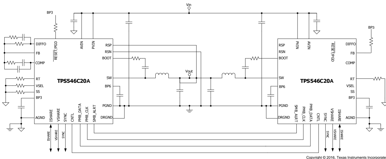
Figure 23. 2-Phase Application
