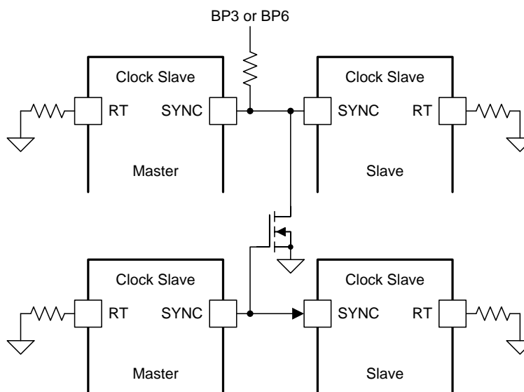
✎ 29. Phase Interleaving Timing
