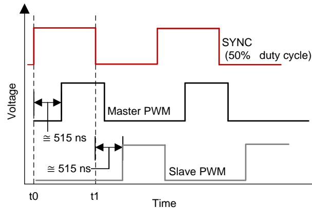
✎ 28. Phase Interleaving Timing
