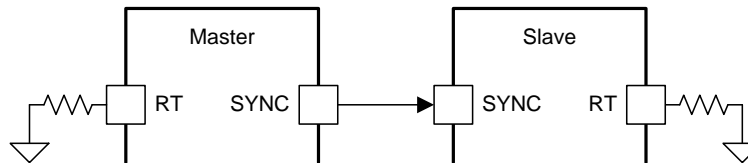
✎ 27. Master-Slave Synchronization and Phase Interleaving Setting
