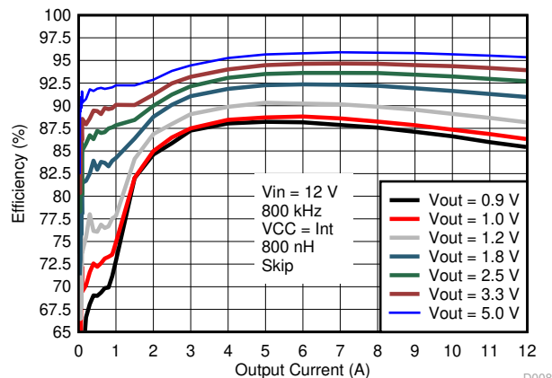
Figure 6-1. Efficiency vs Output Current, Skip-mode, Internal VCC LDO
