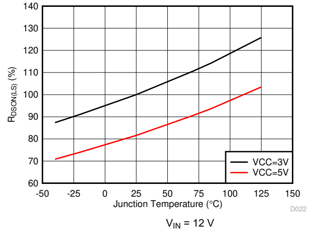
6-14. R_{DS(on)(LS)} vs Junction Temperature
