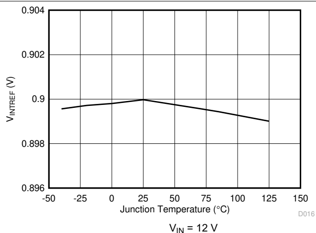
6-10. V_{INTREF} vs Junction Temperature
