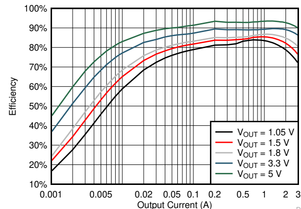
TPS563201 Efficiency
