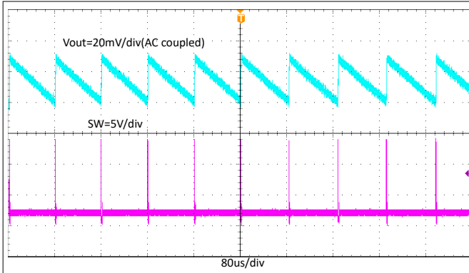
8-8. TPS565242 Output Voltage Ripple with 0.01-A Loading
