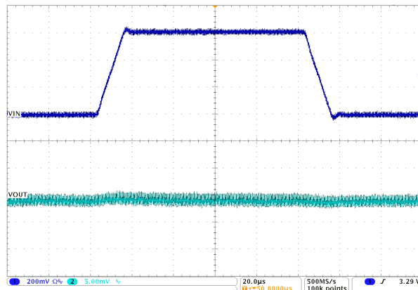
10-13. Line Transient Response
