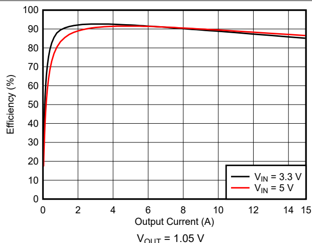
10-10. Efficiency
