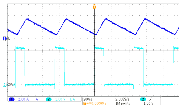
10-15. PWM-CCM Operation
