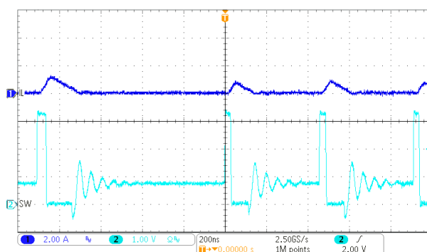
10-17. PFM Operation
