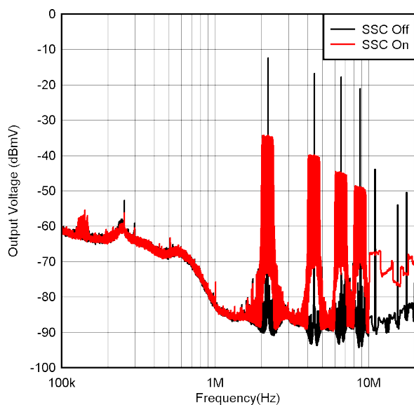
10-18. Spread Spectrum Operation
