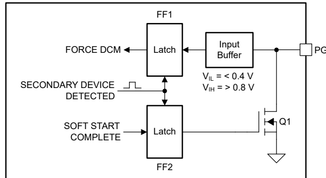
9-13. Power-Good Functional Block Diagram (Secondary Device)
