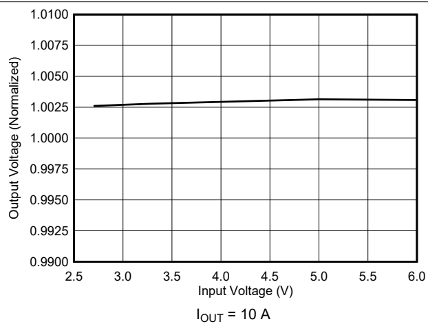
10-12. Line Regulation
