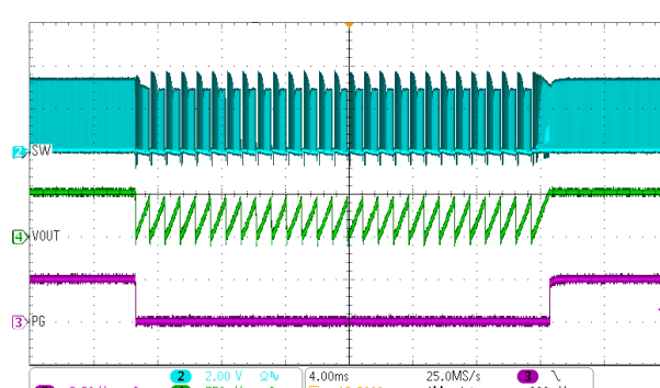
10-23. Current Limit (Hiccup)
