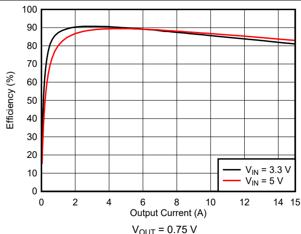
10-6. Efficiency
