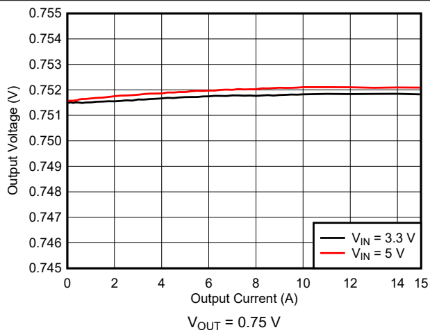
10-7. Load Regulation
