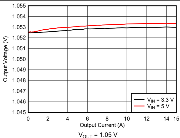
10-11. Load Regulation
