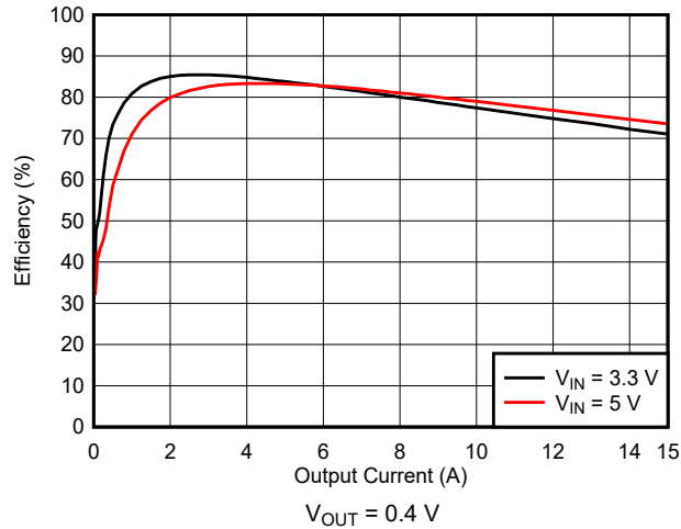
図 10-2. Efficiency
