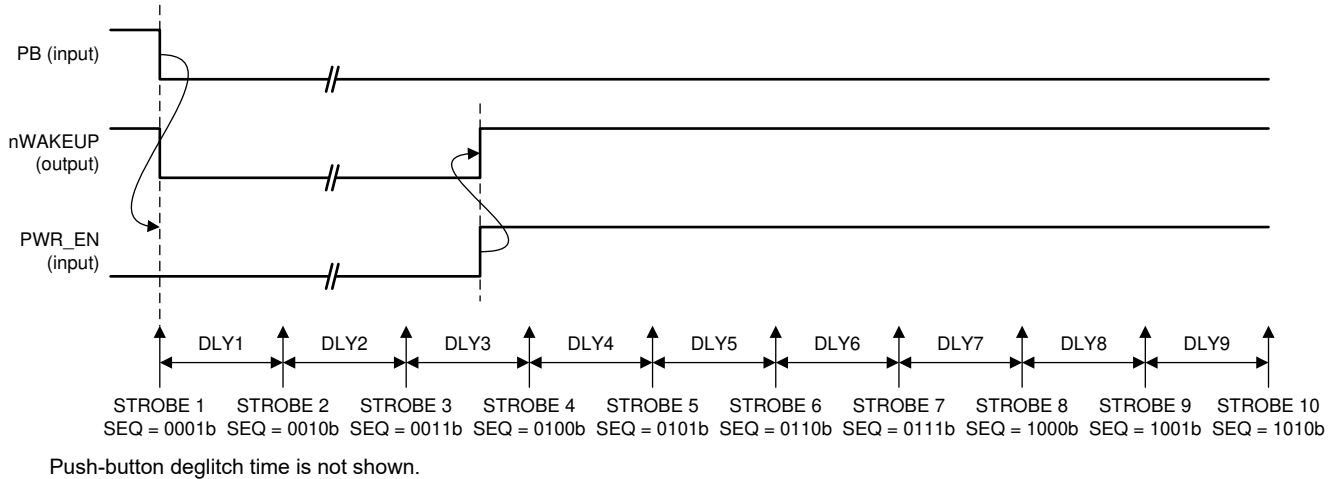
8-1. Power-Up Sequences from OFF or SUSPEND State; PB is Power-Up Event
