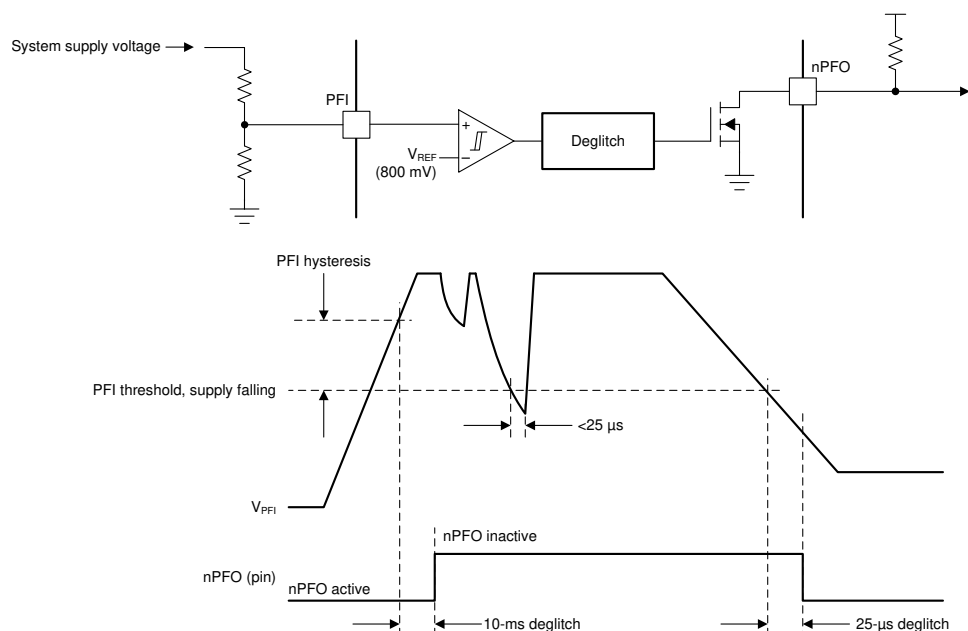
FIG 8-16. Power-Fail Comparator Simplified Circuit and Timing Diagram
