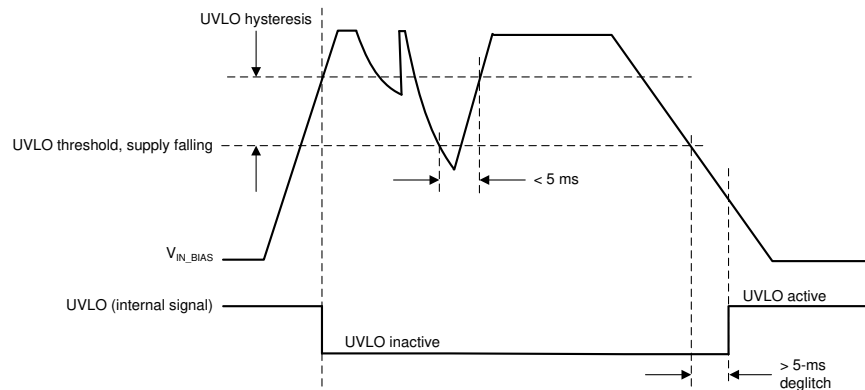
FIG 8-15. Definition of UVLO and Hysteresis
