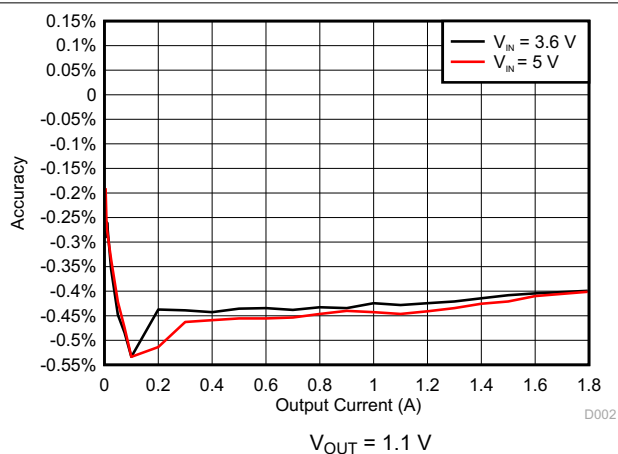
7-2. DCDC2 Accuracy
