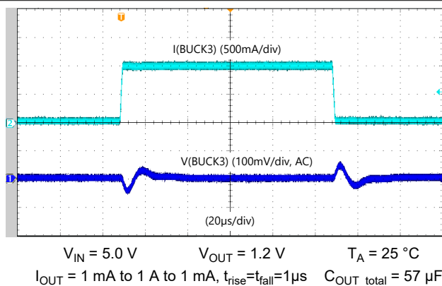
图 6-5. BUCK3 Load-step response - Low Bandwidth, forced PWM
