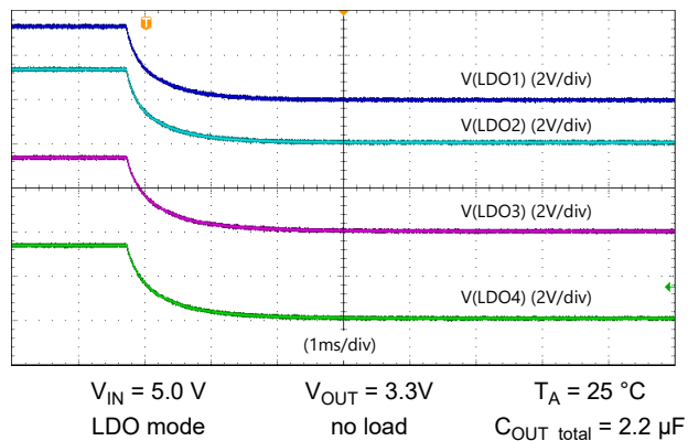
8-16. LDOs Discharge
