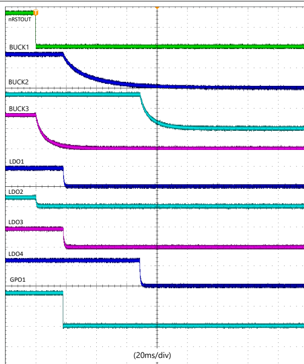
8-16. LDOs Discharge
