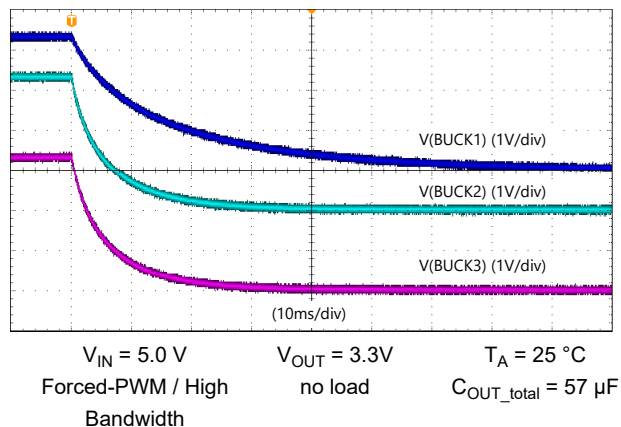
8-15. Bucks Discharge
