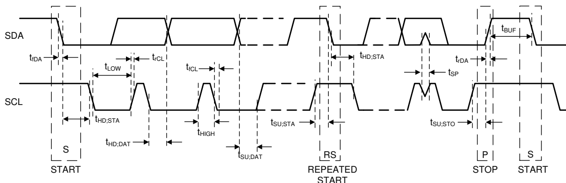
FIG 7-6. I 2 C-Compatible Timing
