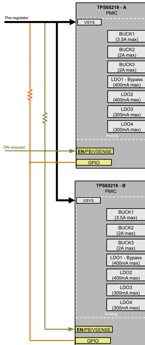
図 8-2. Multi-PMIC Configuration Example
