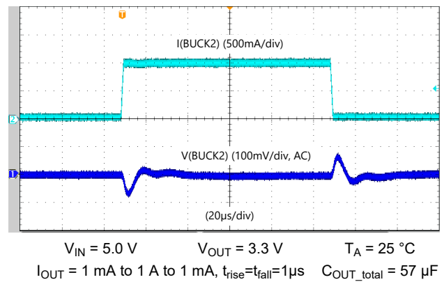
图 6-4. BUCK2 Load-step response - Low Bandwidth, forced PWM
