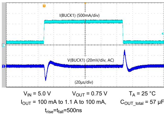
图 6-3. BUCK1 Load-step response - High Bandwidth, forced PWM
