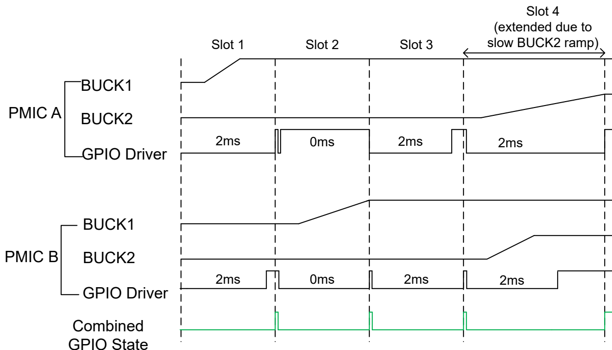
图 8-4. Synchronization during power-up sequence
