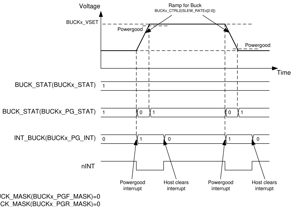
Figure 9. Regulator Output Voltage Change
