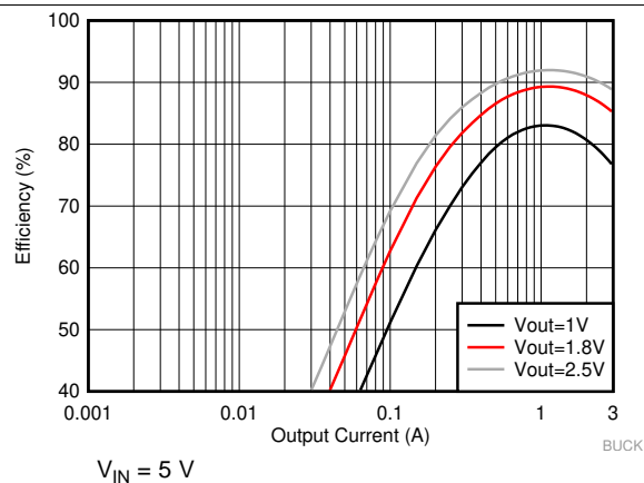
Figure 25. Buck Efficiency in Forced PWM Mode
