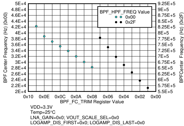
6-11. Receive Signal Path Bandpass Filter Center Frequency Trim
