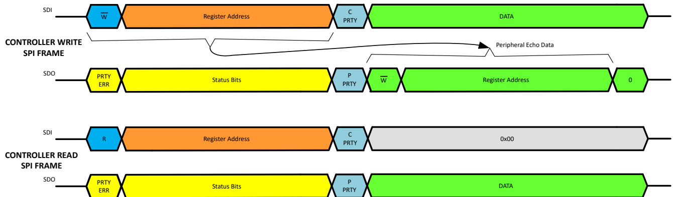
图 7-9. SPI Transfer Sequence
