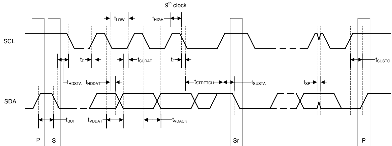
✎ 1. I 2 C Timing Diagram
