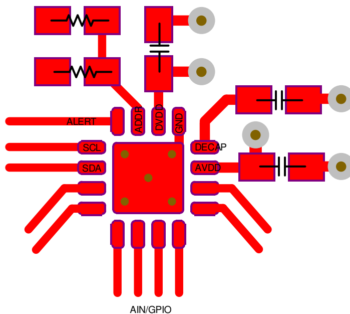
Figure 141. Example Layout
