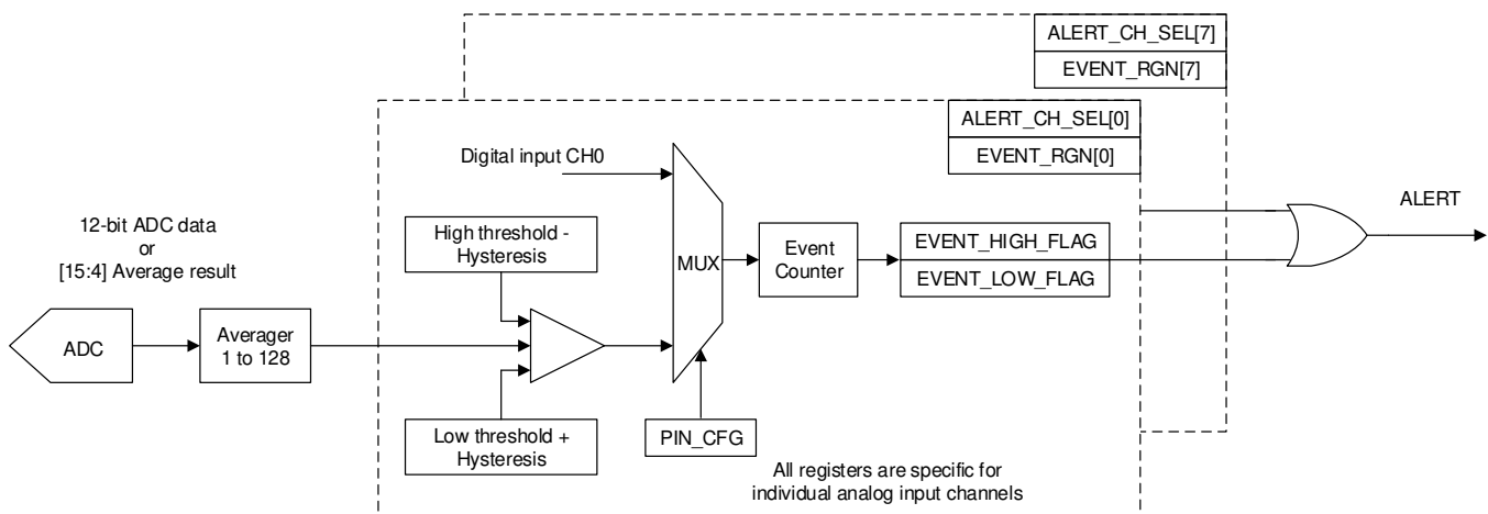
Figure 7. Digital Window Comparator Block Diagram
