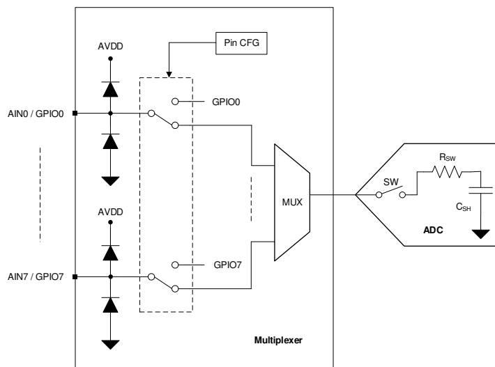
Figure 2. Analog Inputs, GPIOs, and ADC Connections
