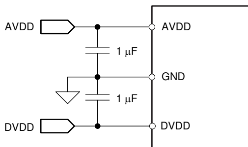
Figure 140. Power-Supply Decoupling
