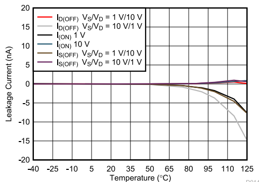
6-13. Leakage Current vs Temperature
