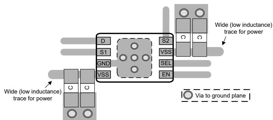
11-3. TMUX7219RQX Layout Example
