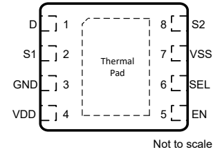
図 5-2. RQX Package, 8-Pin WSON (Top View)
