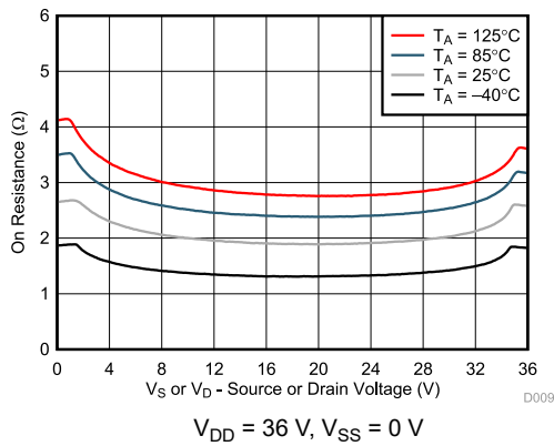
Figure 6-9. On-Resistance vs Temperature
