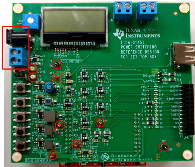
図 6. Board Image With TP Highlighted and Items Relevant to Setup
