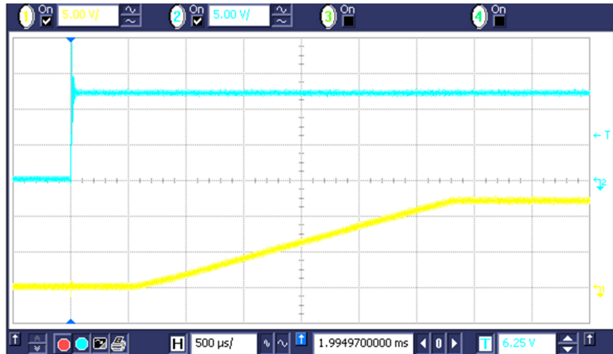
Figure 20. Hot Plug Event on eFuse
