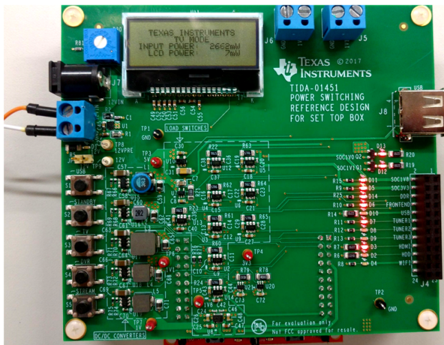
図 12. TV Button LEDs (HDMI, Tuner1, Front End, SOC+DDR)
