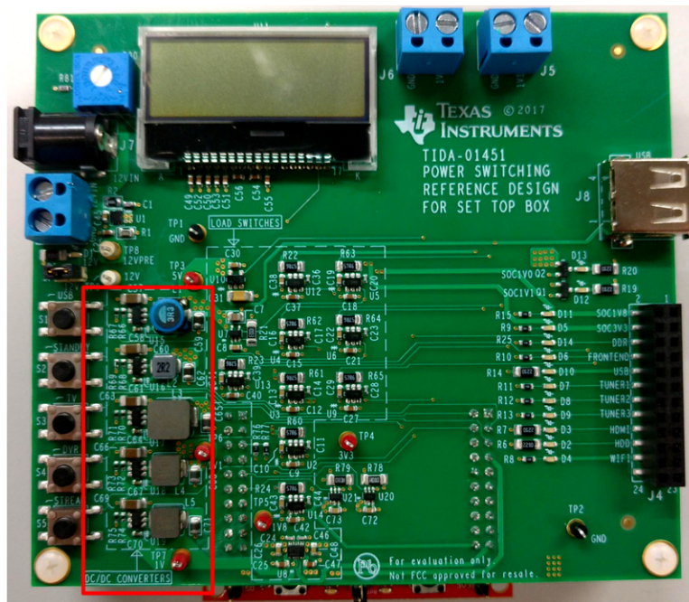
図 3. eFuse and DC/DCs
