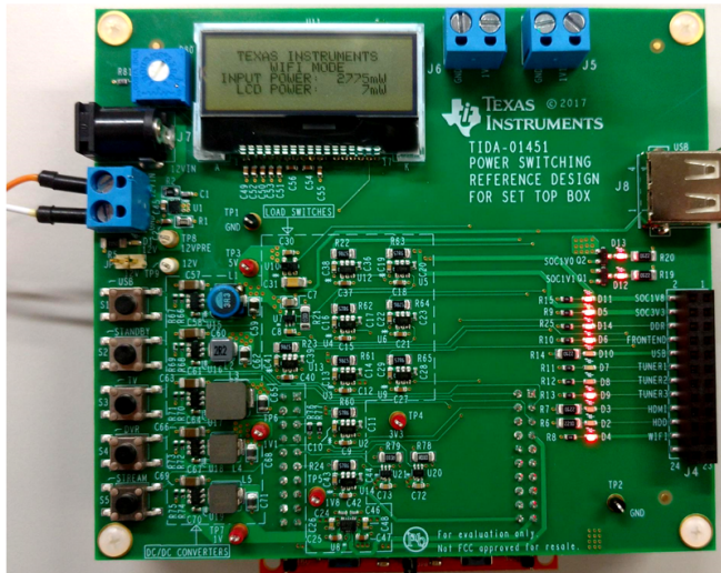
☒ 14. Stream Button LEDs (WIFI, Tuner3, Front End, SOC+DDR)
