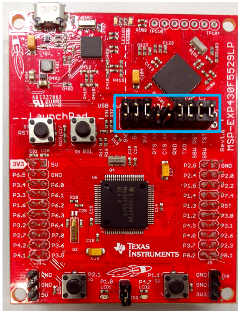
図 5. MSP430™ LaunchPad™ Jumpers to Remove
