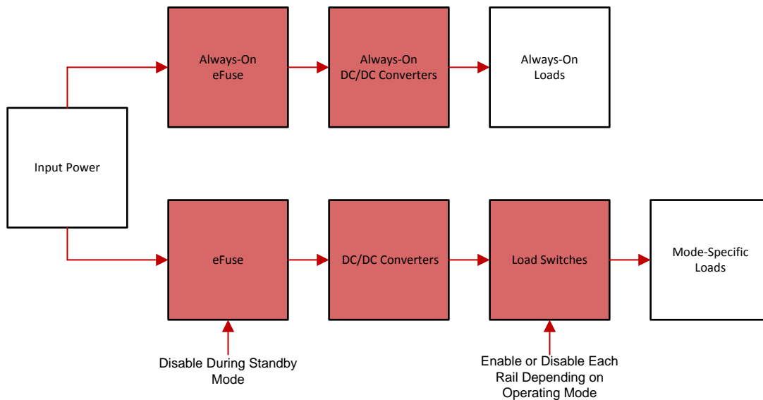
図 4. Separate Always-On Power Tree for Additional Power Savings
