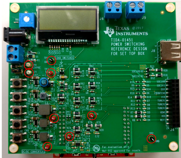
図 18. Board Image With Test Points Highlighted
