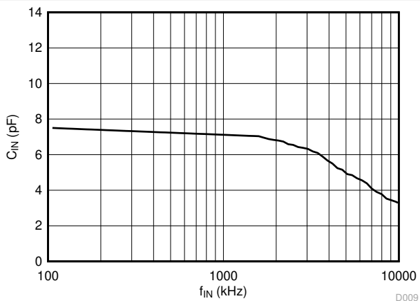
Figure 6-8. Input Capacitance vs Input Signal Frequency
