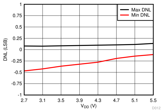
REF-DIV = 0 and BUFF-GAIN = 0 Figure 7-14. Differential Linearity Error vs Supply Voltage
