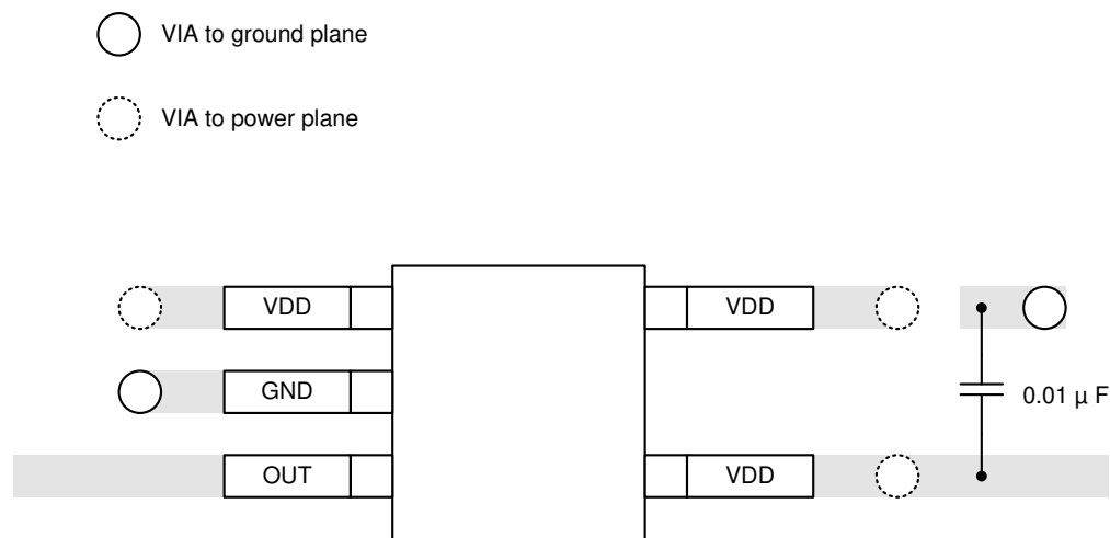
Figure 11-1. SC70 Package Recommended Layout
