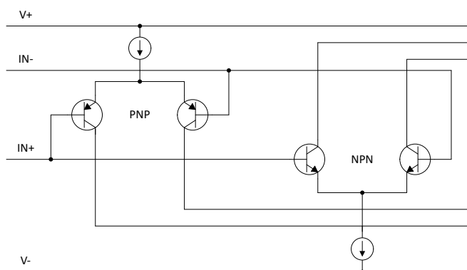
Figure 6-2. Rail-to-Rail Input Stage
