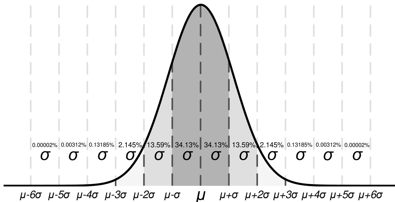
Figure 6-5. Ideal Gaussian Distribution
