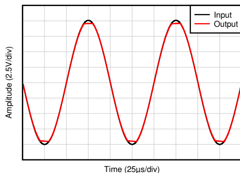
Figure 6-3. No Phase Reversal
