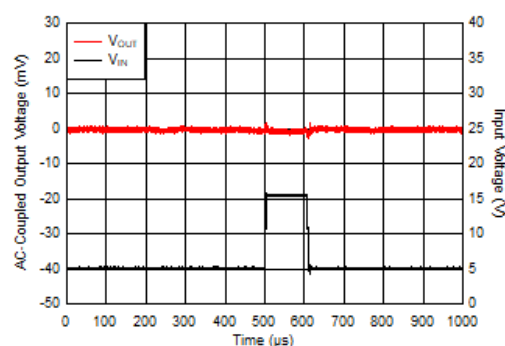
Figure 5-10. V_{IN} Transient From 5 V to 16 V
