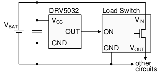
Figure 4. Typical Load Switch Schematic
