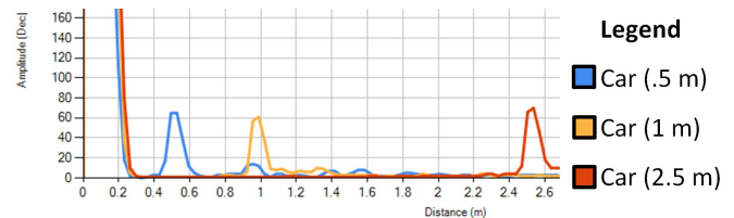
Figure 5. Vehicle Detection For Garage Gate
