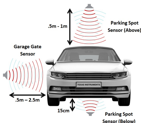
Figure 2. Mounting for Vehicle Detection
