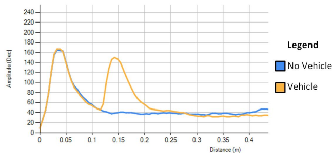
Figure 3. Occupancy Detection Below Vehicle
