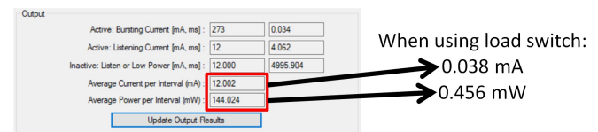
Figure 6. Power Optimization
