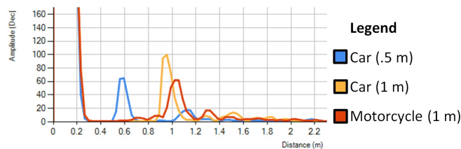
Figure 4. Occupancy Detection Above Vehicle
