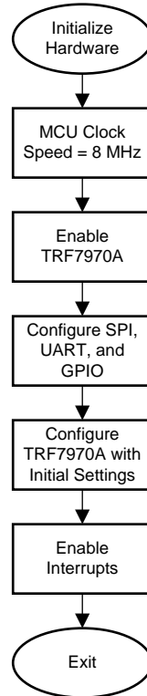
Figure 6. Hardware Initialization Flowchart
