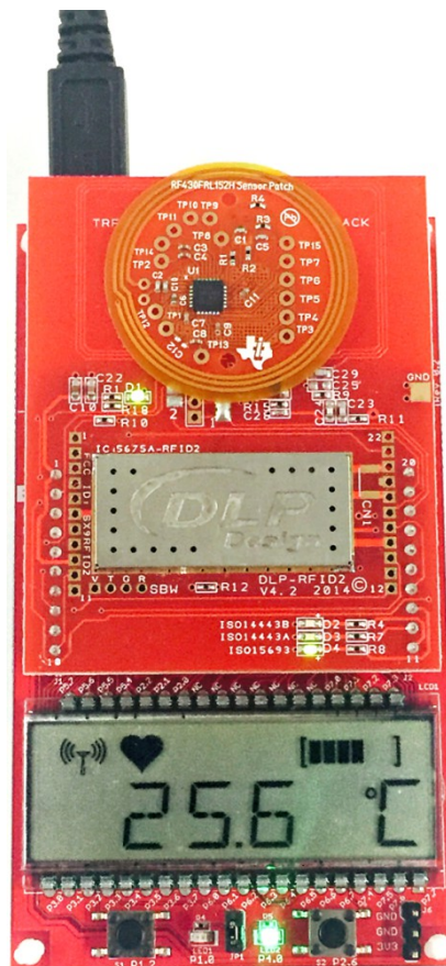
Figure 1. RF430FRL152H Sensor Tag and MSP430FR4133 Reader
