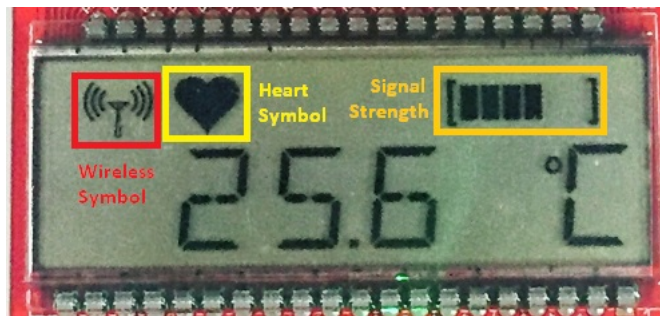
Figure 2. Additional LCD Display Features
