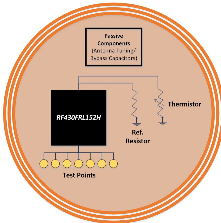
Figure 3. Block Diagram for RF430FRL152 Sensor Tag
