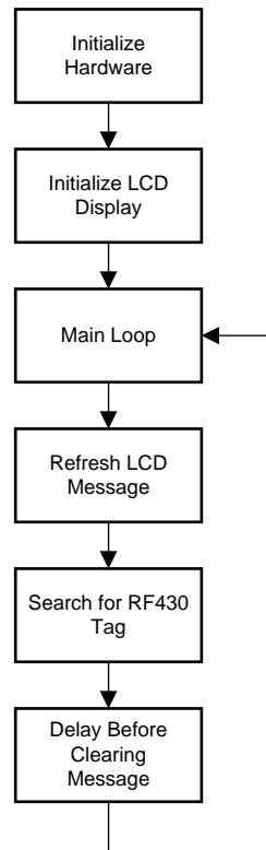
Figure 5. Main.c Flowchart
