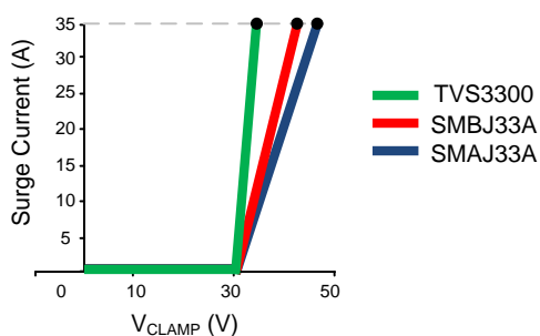
Figure 1. Different Diode IV curves
