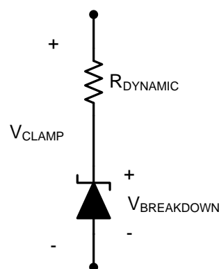
Figure 2. TVS Diode Characteristics
