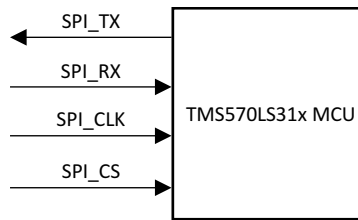
Figure 1. SPI Connections for TMS570LS31x Bootloader
