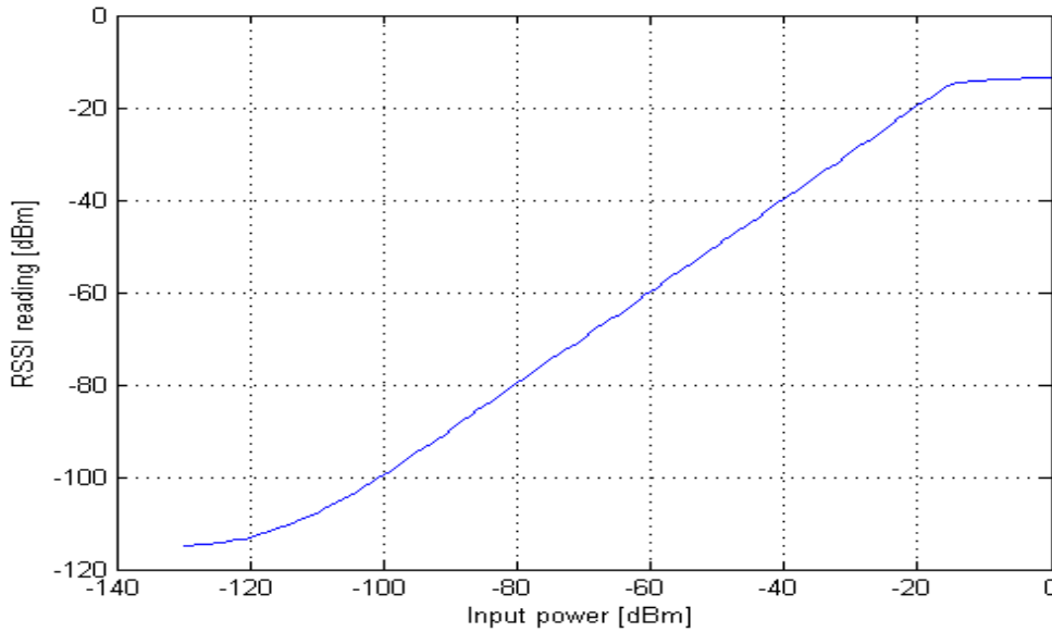
Figure 11. Typical RSSI vs. Input Power Level, HGM, 1.2 kbps, 20 kHz RX BW
