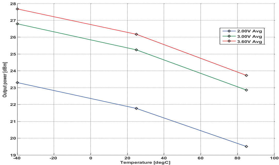
Figure 14. Typical Output Power vs. Temperature and Power Supply Voltage. PA_CFG2 = 0x6B
