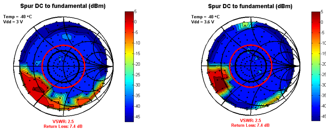
Figure 20. Spurious Frequency Components vs. Load Impedance at SMA Connector at -40°C. PA_CFG2 = 0x6B
