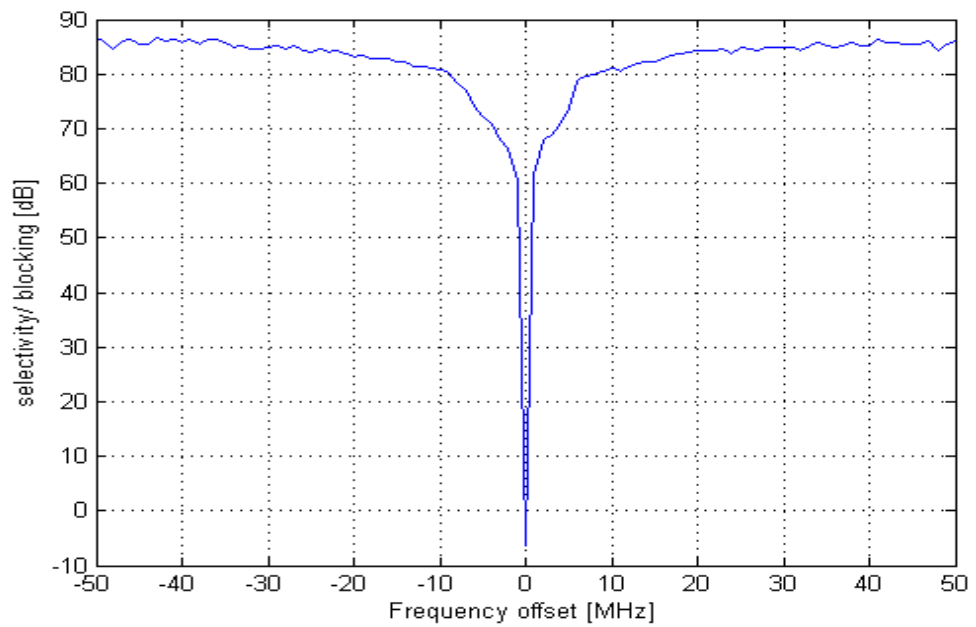
Figure 9. Typical Blocking, 50 kbps
