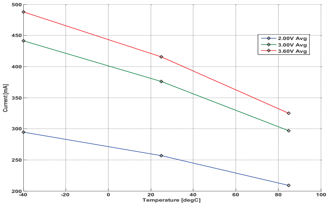
Figure 16. Typical TX Current Consumption vs. Temperature and Power Supply Voltage. PA_CFG2 = 0x6B
