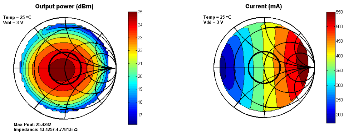
Figure 18. Output Power (left) and Current (right) vs. Load Impedance at SMA Connector at 25°C. PA_CFG2 = 0x6B
