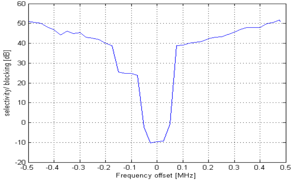
Figure 10. Typical Selectivity, 50 kbps
