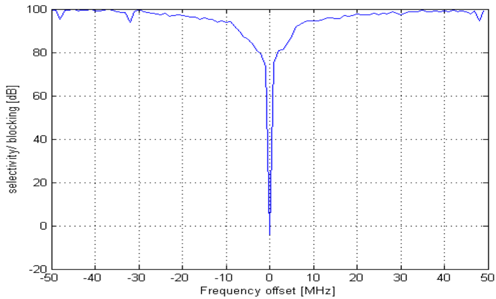
Figure 7. Typical Blocking, 1.2 kbps
