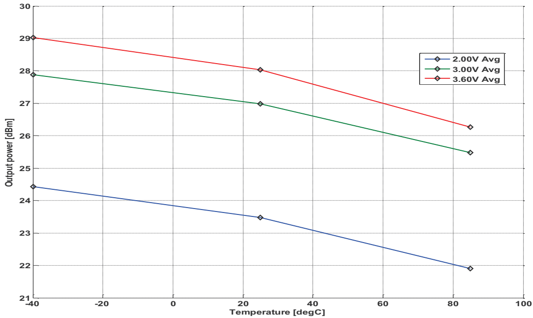
Figure 13. Typical Output Power vs. Temperature and Power Supply Voltage. PA_CFG2 = 0x77
