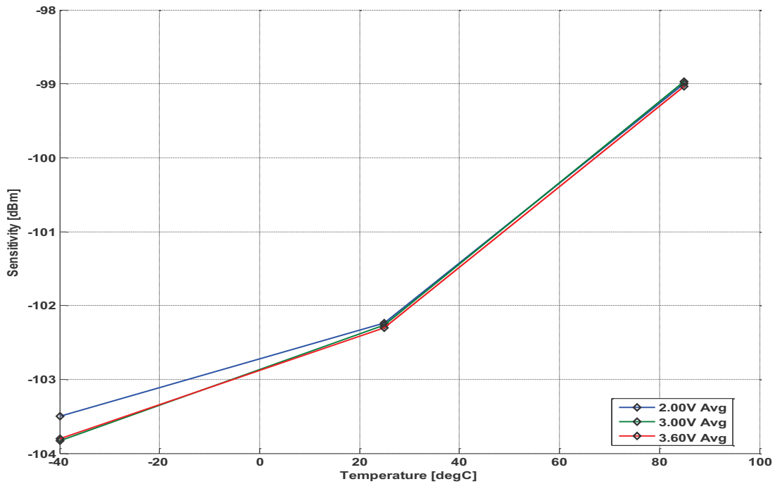
Figure 5. Typical Sensitivity vs. Temperature and Power Supply Voltage, LGM, 50 kbps
