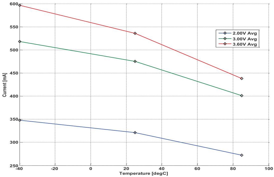
Figure 15. Typical TX Current Consumption vs. Temperature and Power Supply Voltage. PA_CFG2 = 0x77
