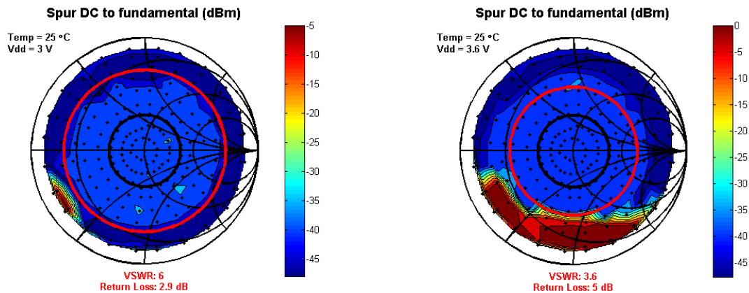
Figure 19. Spurious Frequency Components vs. Load Impedance at SMA Connector at 25°C. PA_CFG2 = 0x6B
