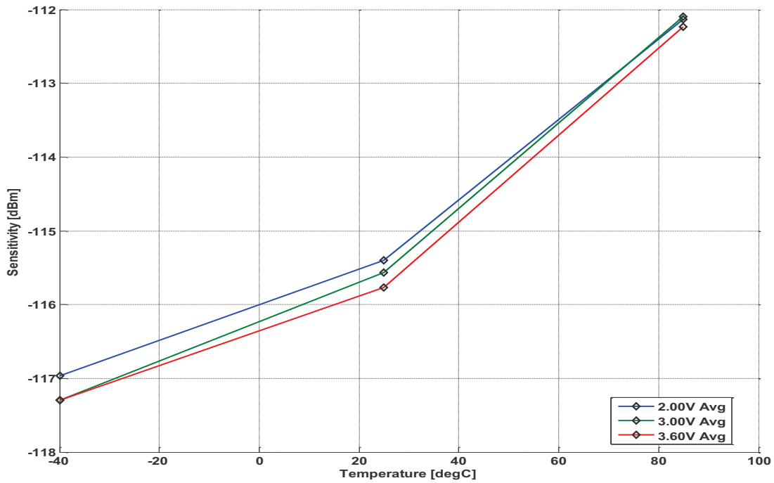
Figure 4. Typical Sensitivity vs. Temperature and Power Supply Voltage, LGM, 1.2 kbps
