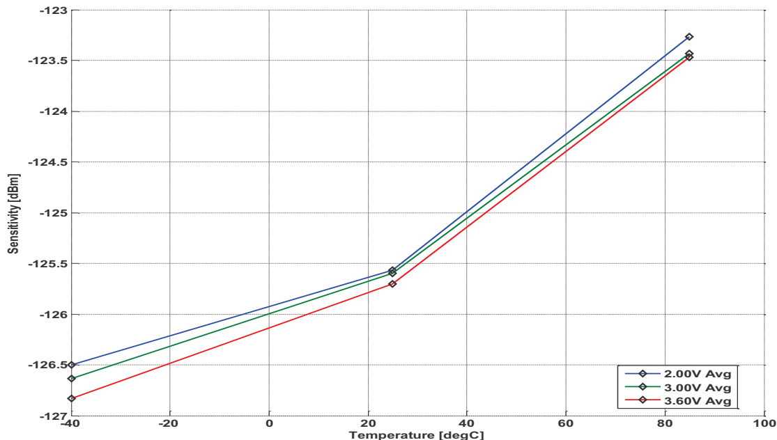
Figure 1. Typical Sensitivity vs. Temperature and Power Supply Voltage, HGM, 1.2 kbps
