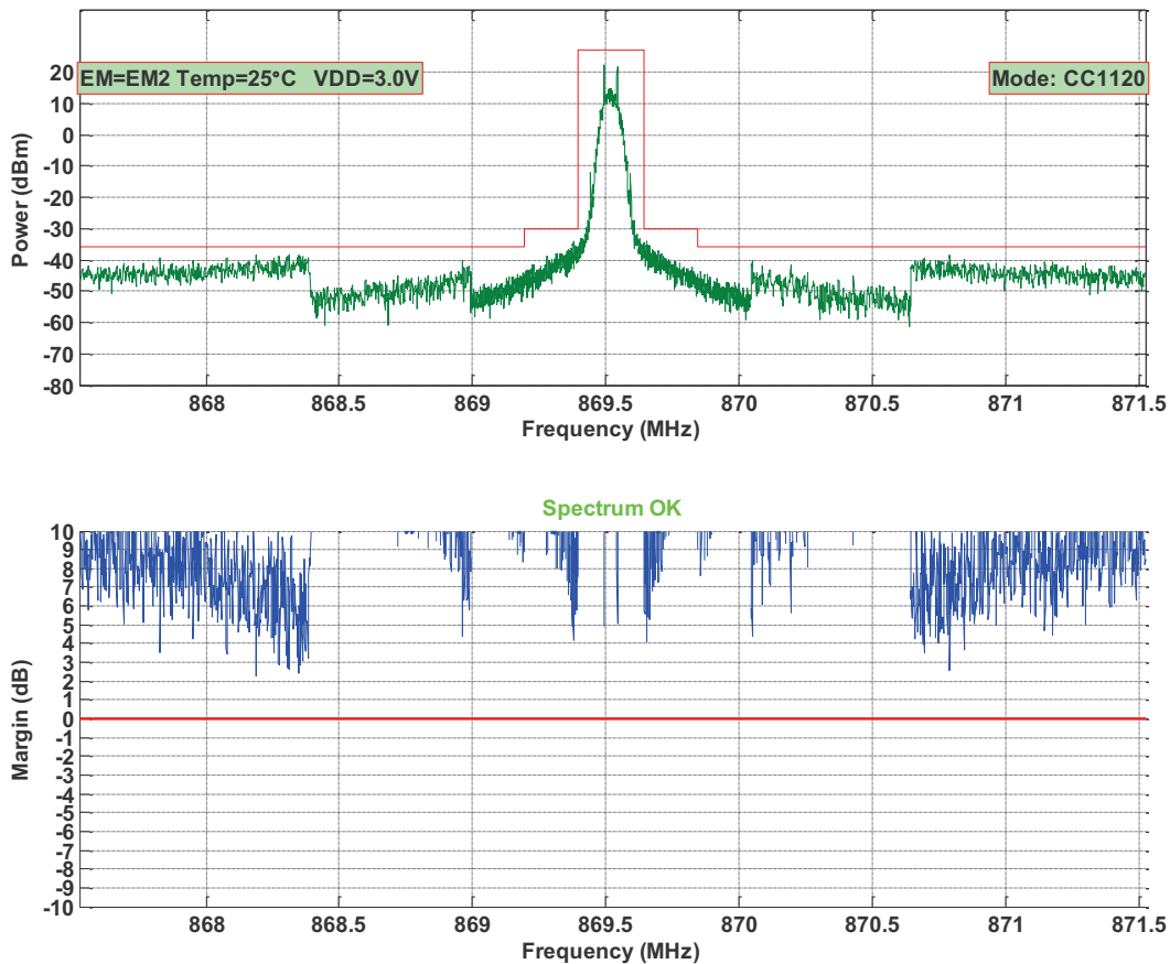
Figure 17. ETSI 300 220, Modulation Bandwidth, Conducted, 50 kbps, PA_CFG2 = 0x77
