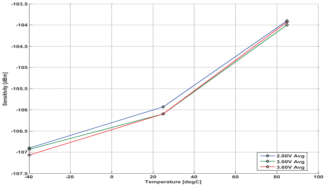
Figure 3. Typical Sensitivity vs. Temperature and Power Supply Voltage, HGM, 200 kbps
