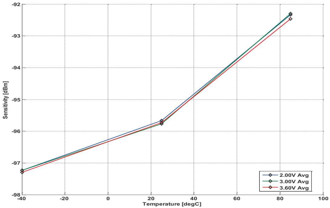
Figure 6. Typical Sensitivity vs. Temperature and Power Supply Voltage, LGM, 200 kbps
