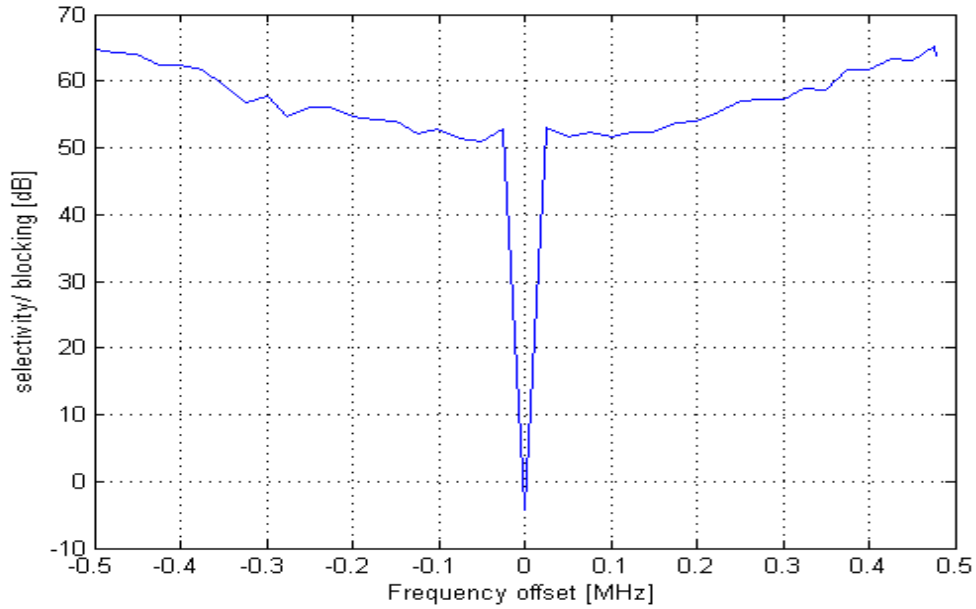
Figure 8. Typical Selectivity, 1.2 kbps
