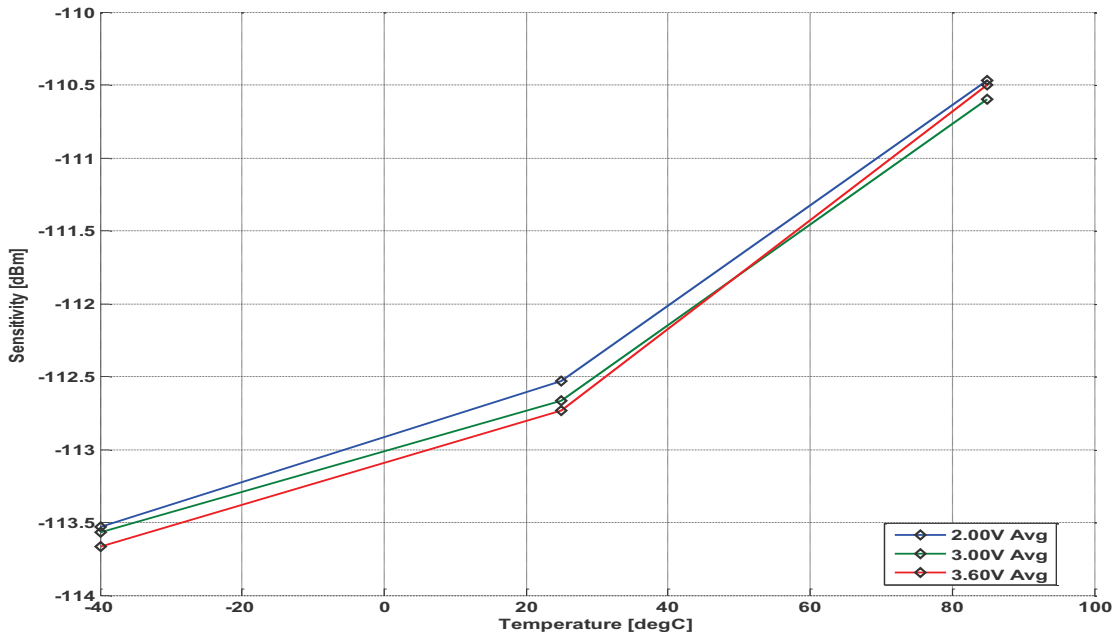
Figure 2. Typical Sensitivity vs. Temperature and Power Supply Voltage, HGM, 50 kbps
