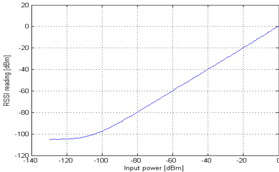
Figure 12. Typical RSSI vs. Input Power Level, LGM, 1.2 kbps, 20 kHz RX BW
