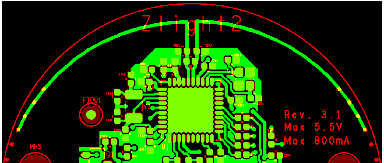
Figure 11. The Final Layout of the Antenna and Filtering Components
