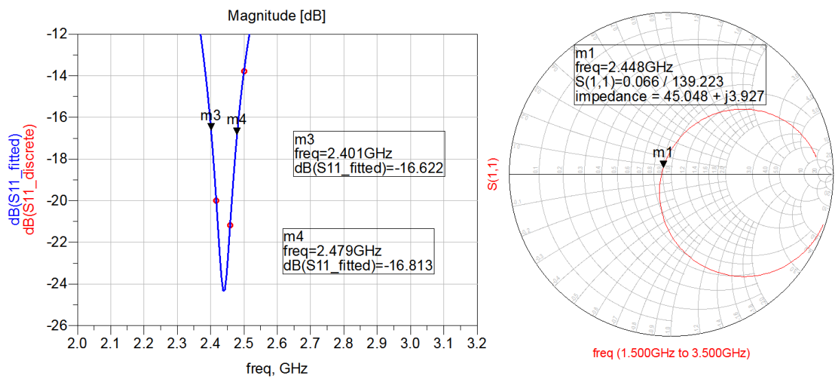
Figure 5. S11 Looking into the Curved Dipole
