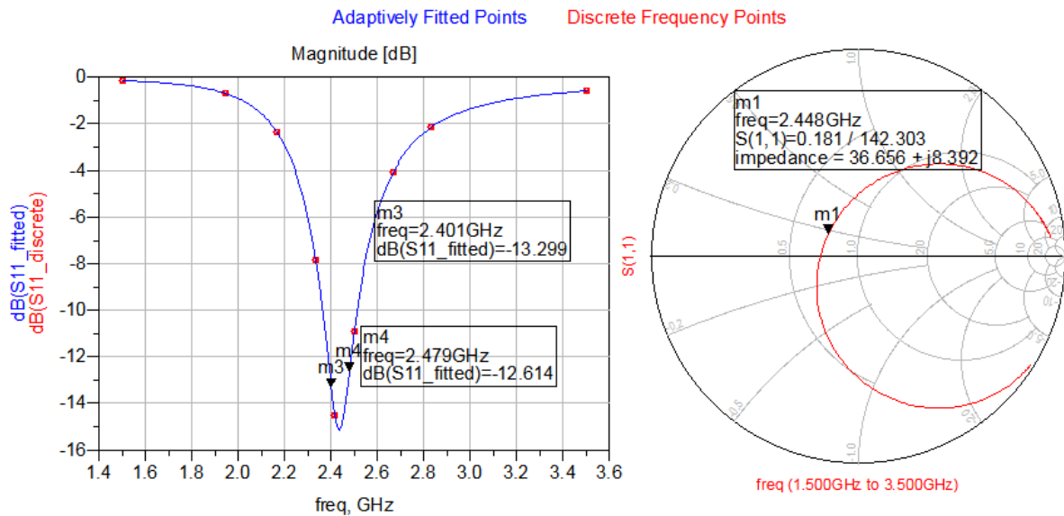
Figure 7. S11 Looking into the Curved Dipole with Added Ground Plane
