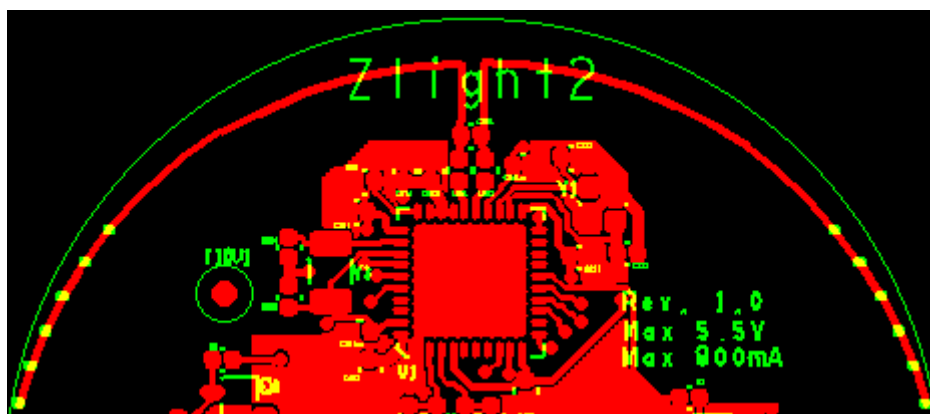
Figure 8. First Prototype Layout with Tuning Marks and Filtering Components
