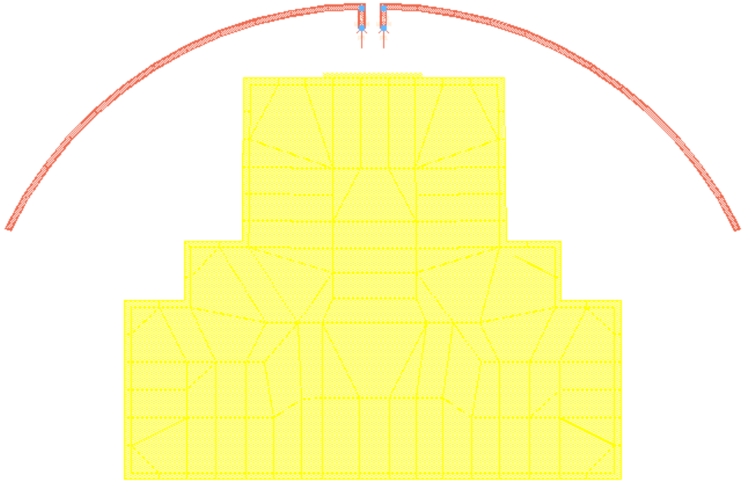
Figure 6. A Ground Plane is Added to Improve the Accuracy of the Board Model
