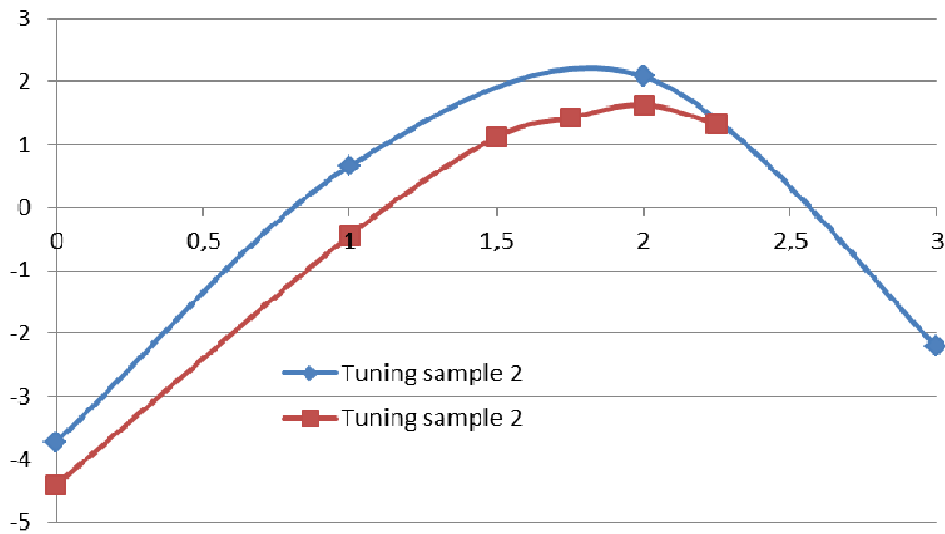
Figure 9. TRP (in dBm) versus the Number of Notches Cut (x-axis)
