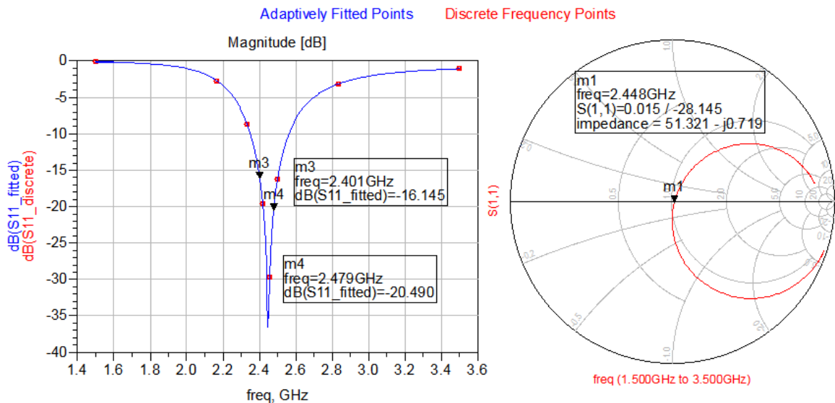
Figure 3. Simulated S11. Substrate: 800 \mu\text{m} FR4
