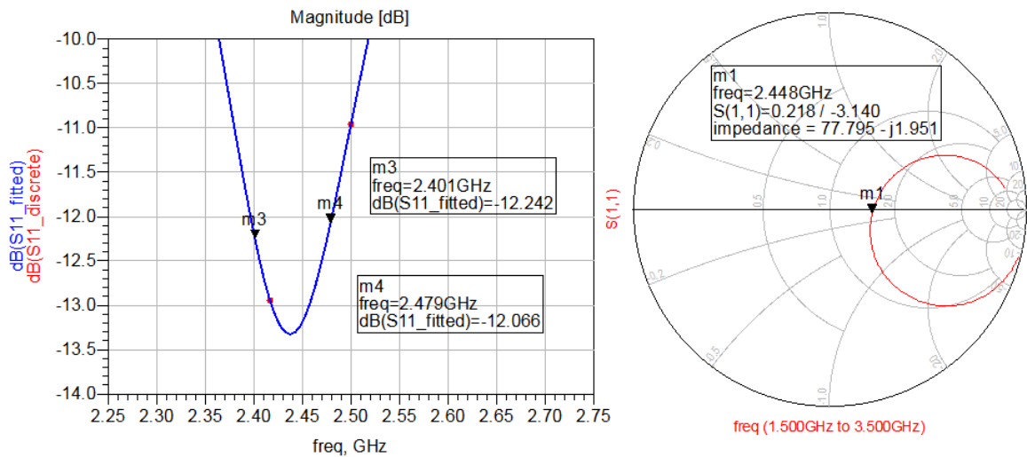
Figure 2. Simulated S11. Substrate: Free Space
