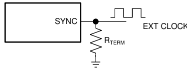
FIG 18. Frequency Synchronization
