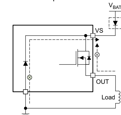
Figure 8-14. Reverse-Current External Protection, Method 1
