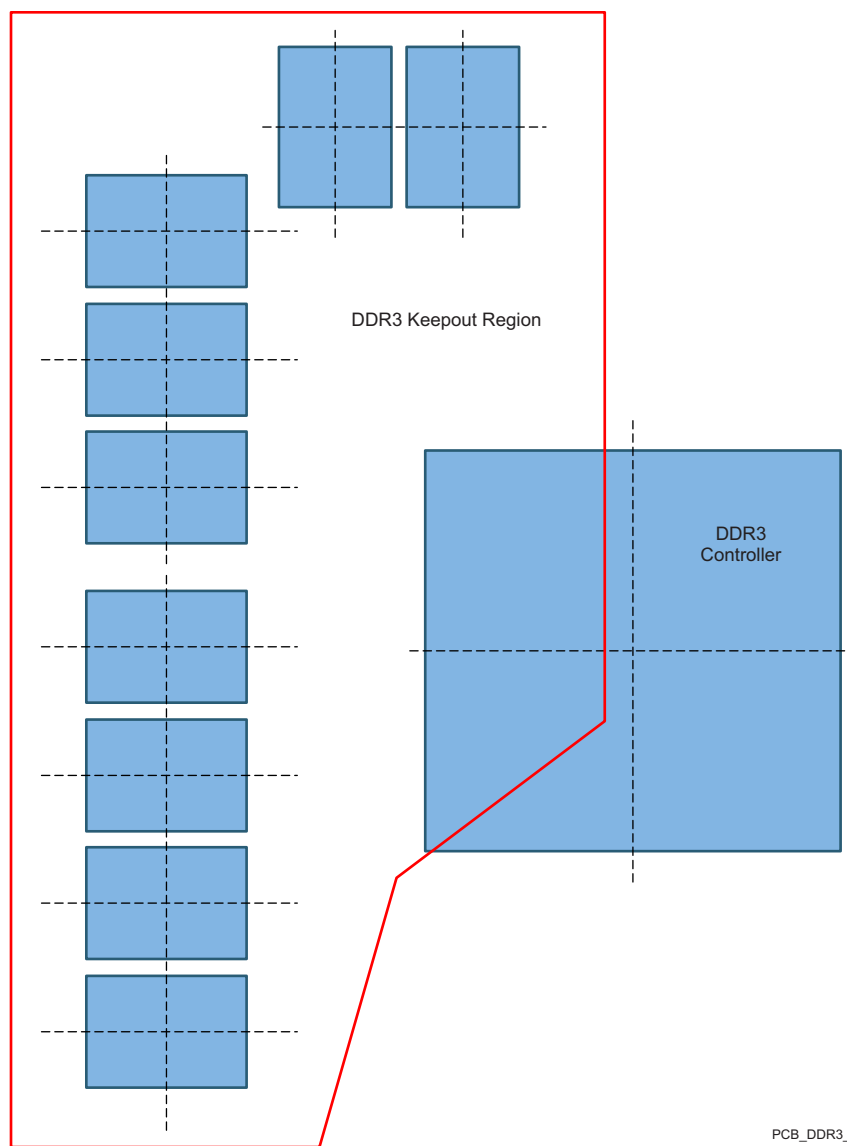
Figure 8-5. DDR3 Keepout Region
