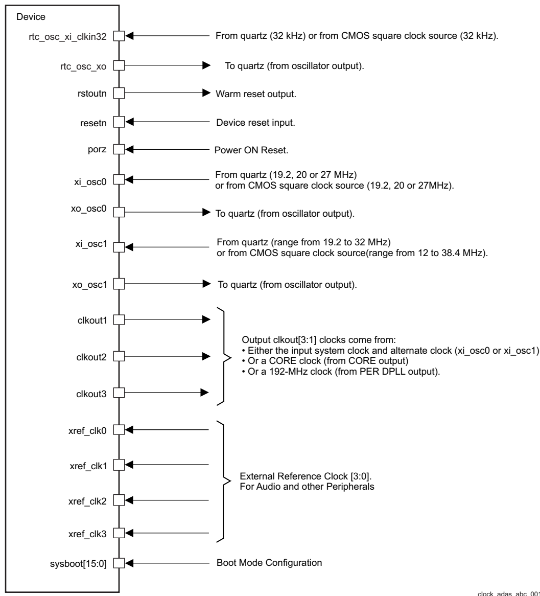
Figure 6-1. Clock Interface
