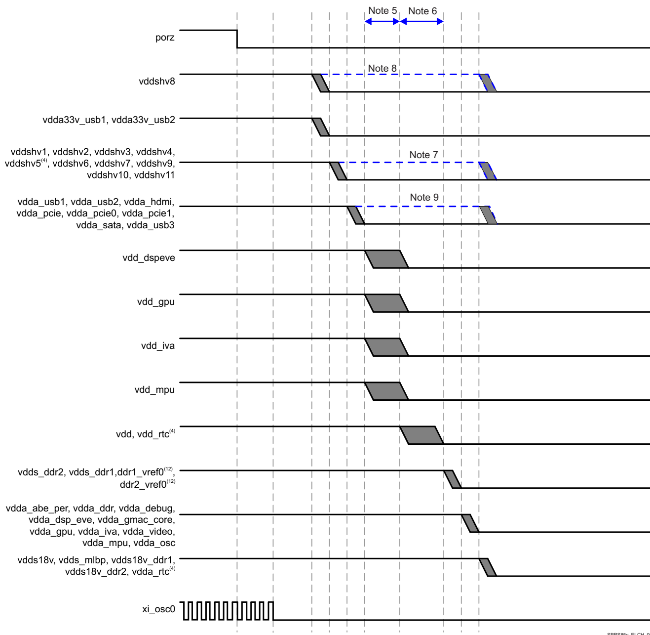
Figure 5-3. Power-Down Sequencing (10)(11)
