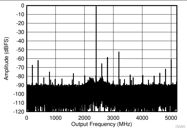
FIG 5-10. DES Mode: Single Tone FFT at 7997 MHz
