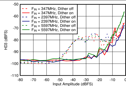
图 5-78. Dual Channel Mode: HD3 vs Input Amplitude and Dither
