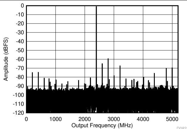
FIG 5-7. DES Mode: Single Tone FFT at 2397 MHz
