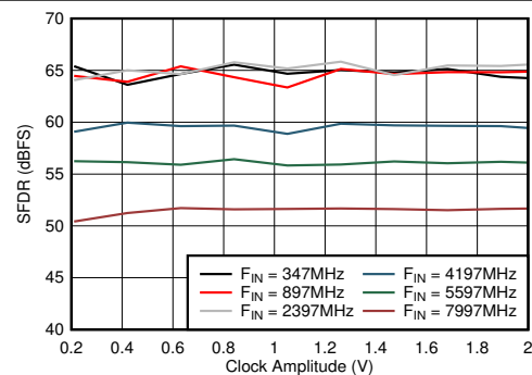
図 5-84. Dual Channel Mode: SFDR vs Clock Amplitude
