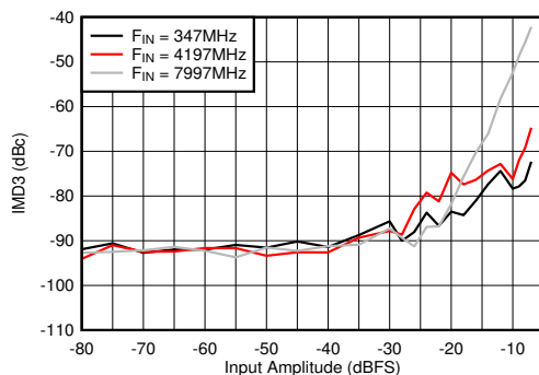
FIG 5-105. Dual Channel Mode: IMD3 vs Input Amplitude
