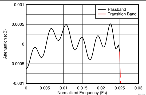
6-16. Decimate-by-16 Composite Zoomed Pass-Band Response
