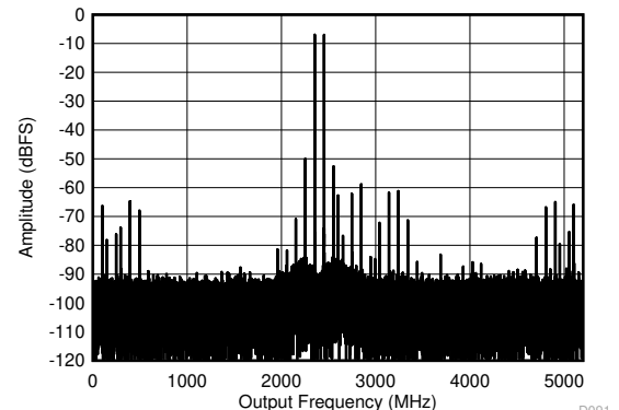
FIG 5-16. DES Mode: Two Tone FFT at 7997 MHz
