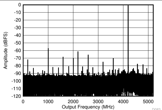
FIG 5-8. DES Mode: Single Tone FFT at 4197 MHz
