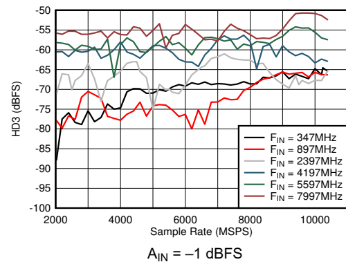
図 5-38. DES Mode: HD3 vs Sample Rate and Input Frequency
