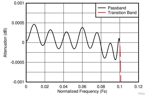
6-12. Decimate-by-4 Composite Zoomed Pass-Band Response
