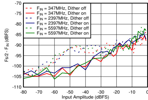
図 5-80. Dual Channel Mode: F_s/2 - F_{\text{IN}} vs Input Amplitude and Dither
