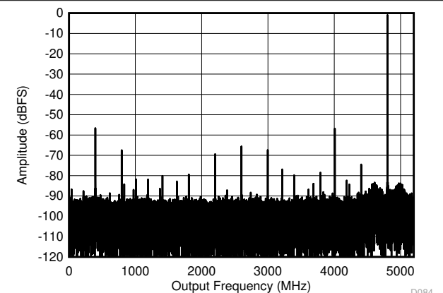
FIG 5-9. DES Mode: Single Tone FFT at 5597 MHz
