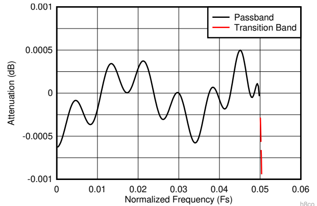
6-14. Decimate-by-8 Composite Zoomed Pass-Band Response
