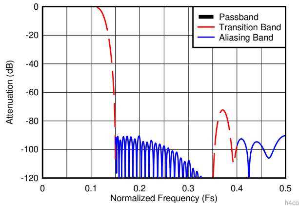
6-11. Decimate-by-4 Composite Response
