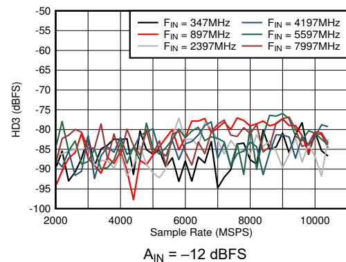
図 5-40. DES Mode: HD3 vs Sample Rate and Input Frequency
