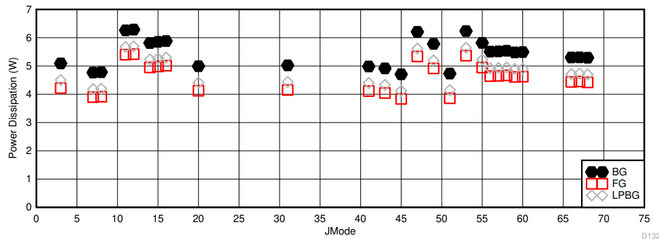
5-115. Dual Channel Mode: I_{D11} vs JMODE at 5.2GSPS
