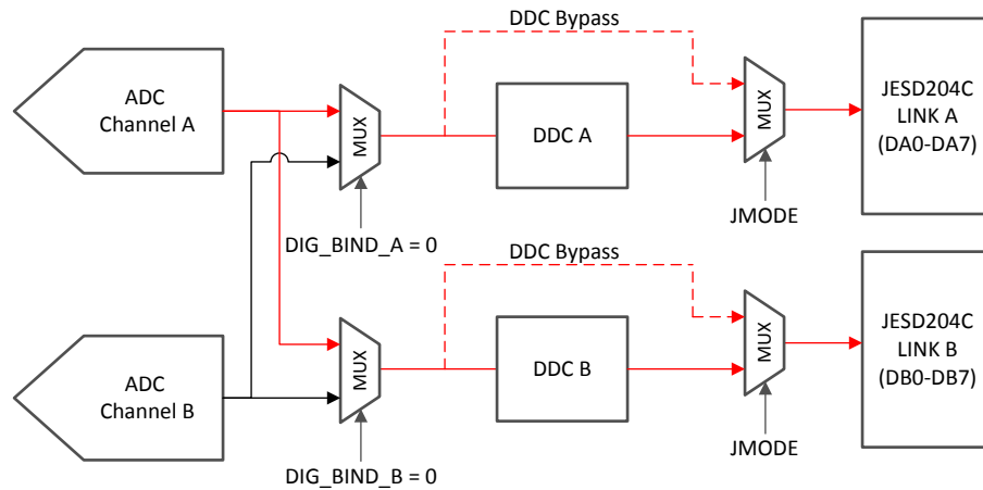
❏ 6-24. Dual DDC Mode or Redundant Data Mode for Channel A
