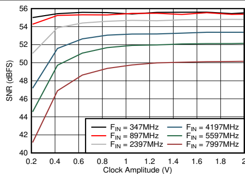
図 5-83. Dual Channel Mode: SNR vs Clock Amplitude
