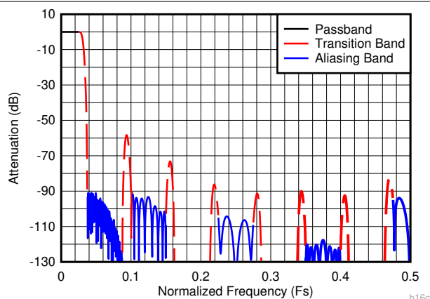
6-15. Decimate-by-16 Composite Response
