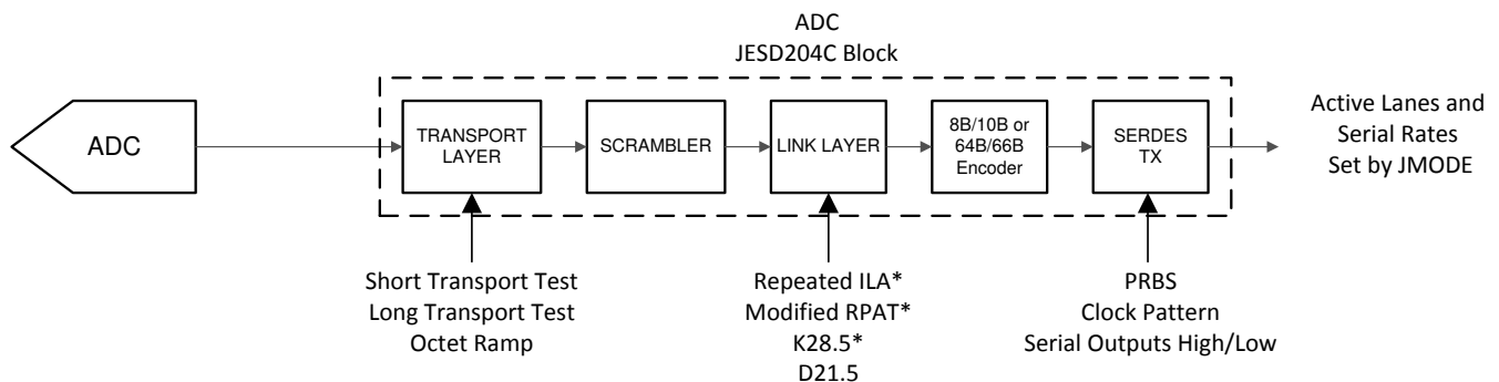
❏ 6-25. Test Mode Insertion Points
