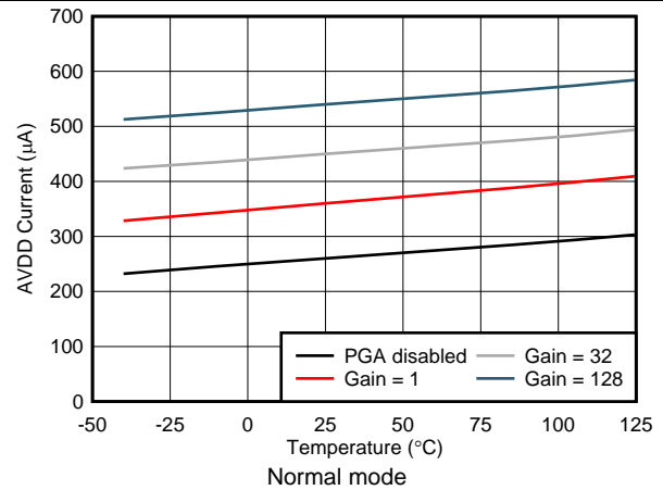
FIG 37. Analog Supply Current vs Temperature
