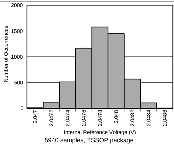
24. Internal Reference Voltage Histogram
