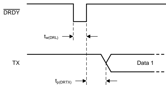
✎ 4. Automatic Data Read Mode \overline{\text{DRDY}} Switching Characteristics
