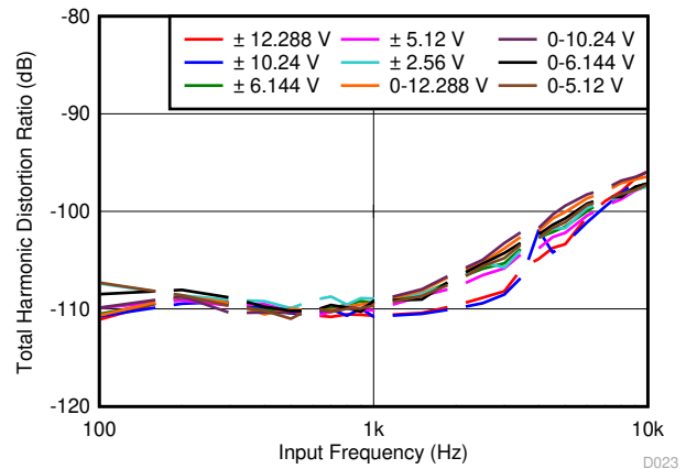
6-40. THD vs Input Frequency
