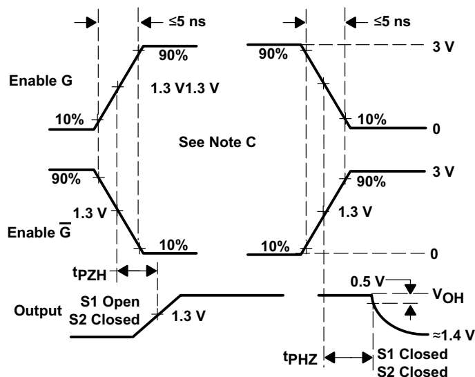
7-3. Voltage Waveforms For t_{PZH} , t_{PHZ}
