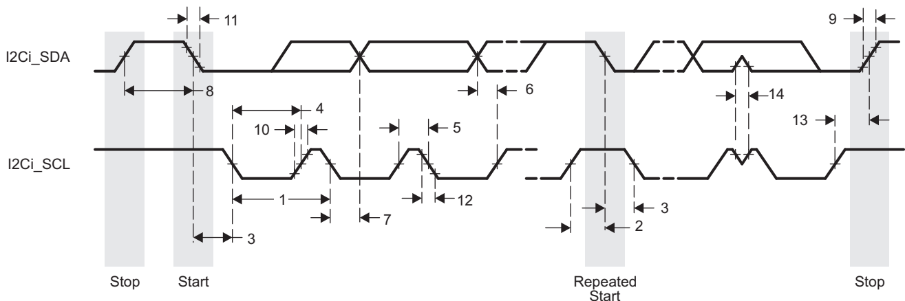
図 5-36. I2C Receive Timing
