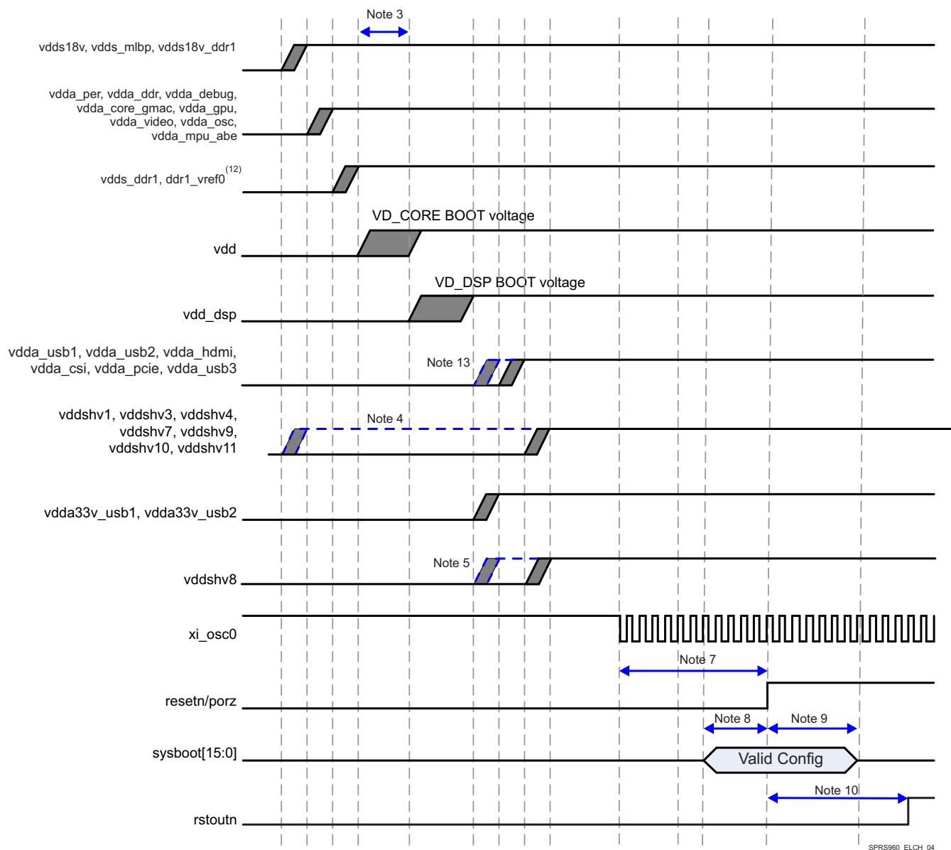
Figure 5-5. Power-Up Sequencing
