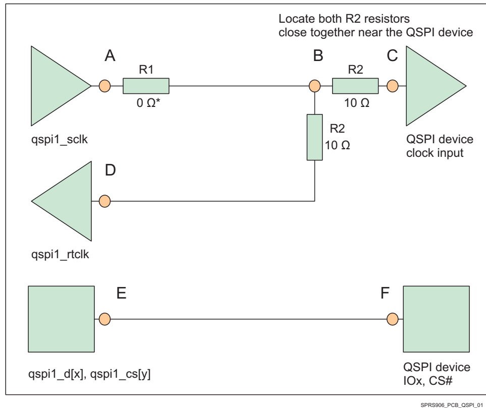
7-30. QSPI Interface High Level Schematic
