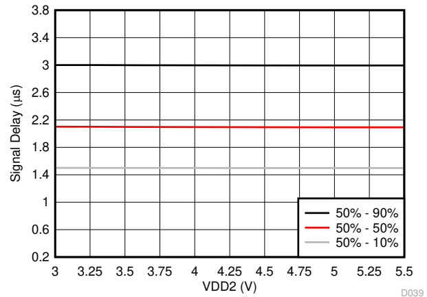
Figure 6-36. IN to OUTP, OUTN Signal Delay vs Low-Side Supply Voltage
