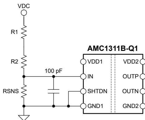
Figure 8-2. Input Filter
