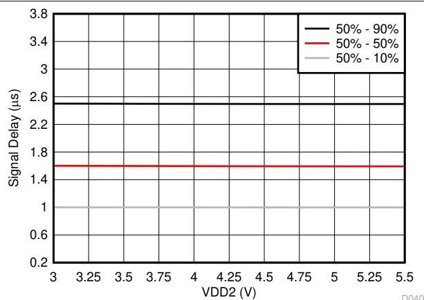
Figure 6-37. IN to OUTP, OUTN Signal Delay vs Low-Side Supply Voltage
