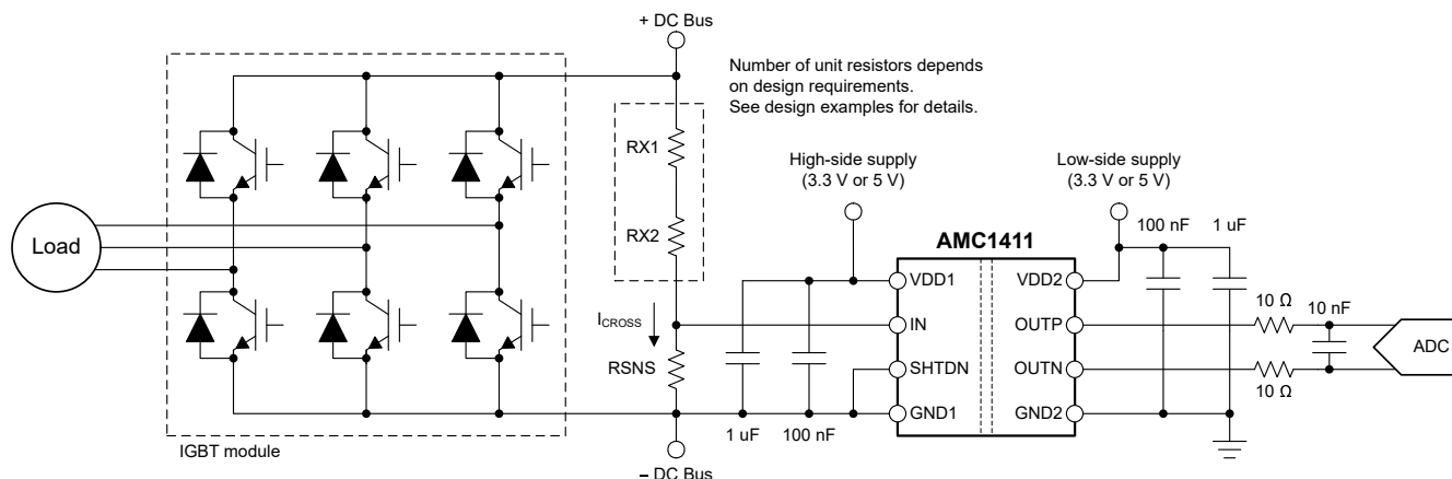
8-1. Using the AMC1411 for DC Link Voltage Sensing in Frequency Inverters
