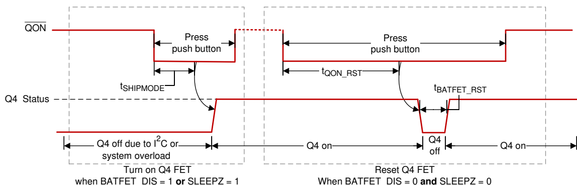
☒ 9-10. \overline{QON} Timing
