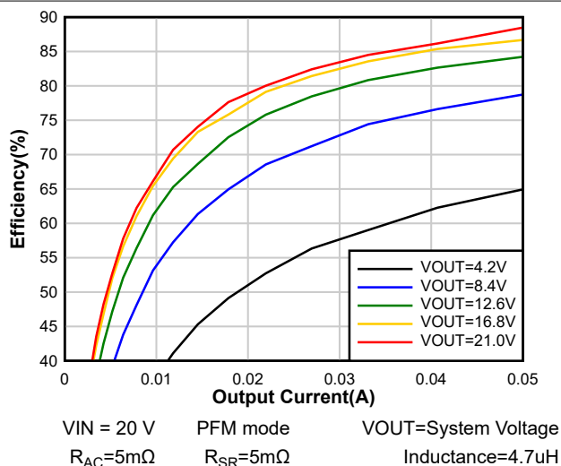
図 7-4. Light Load System Efficiency
