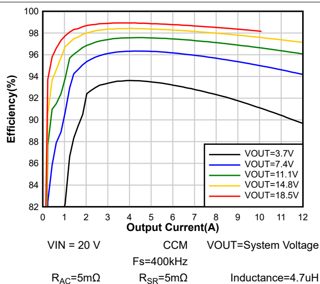
図 7-8. System Efficiency
