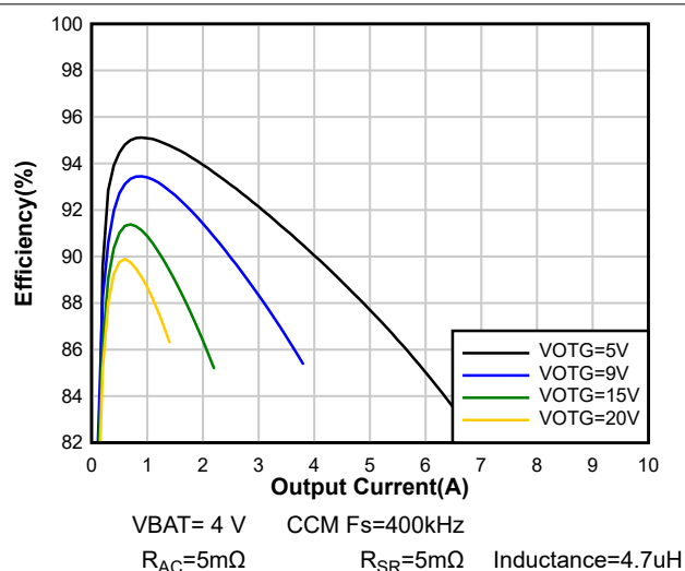
図 7-10. OTG Efficiency with 1S Battery
