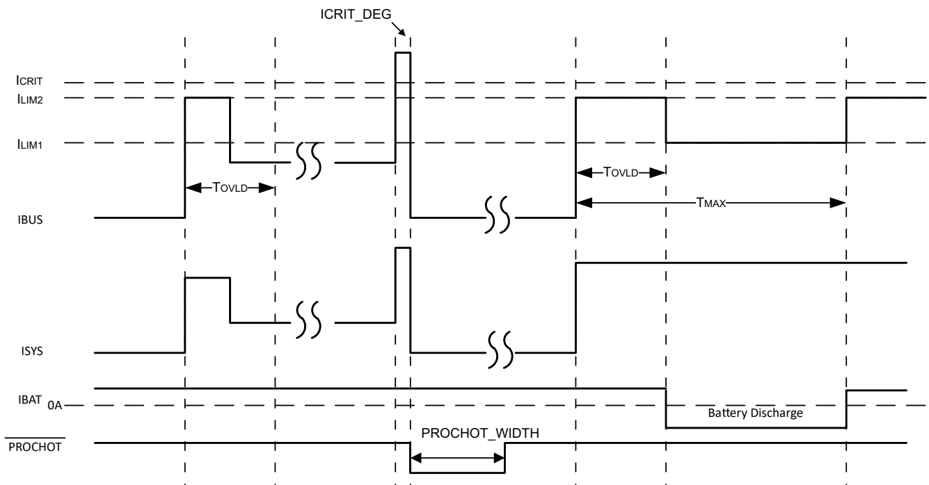
図 8-3. Two-Level Adapter Current Limit Timing Diagram
