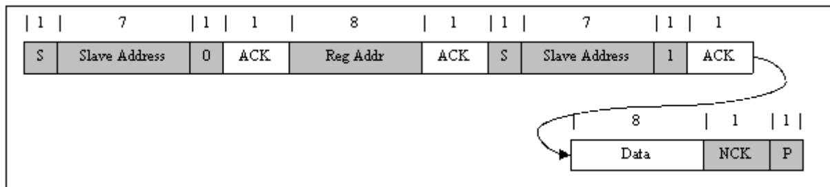
図 8-13. Single Read
