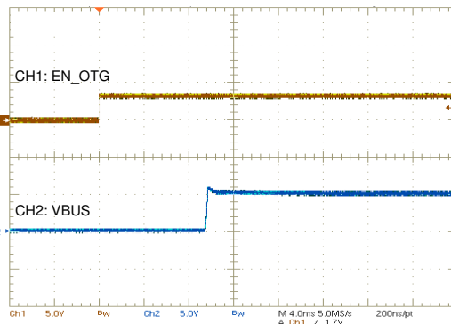
図 9-17. OTG Power Up from 8-V Battery
