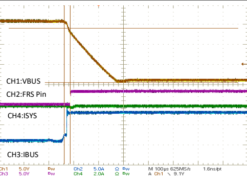
図 9-21. FRS Transition Waveform
