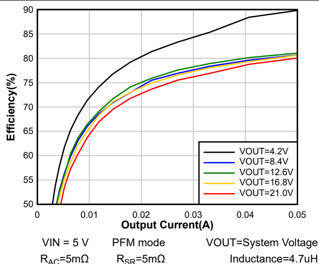
図 7-1. Light Load System Efficiency
