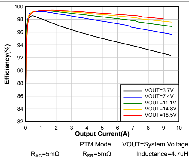
図 7-9. PTM Mode System Efficiency
