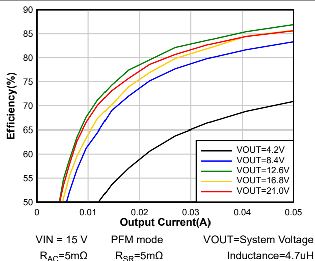
図 7-3. Light Load System Efficiency
