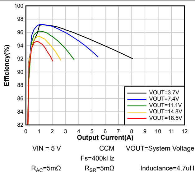
図 7-5. System Efficiency
