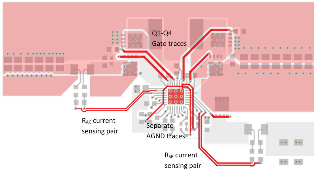
図 11-2. Buck-Boost Charger Gate Drive/Current Sensing/AGND Signal Layer Routing Example
