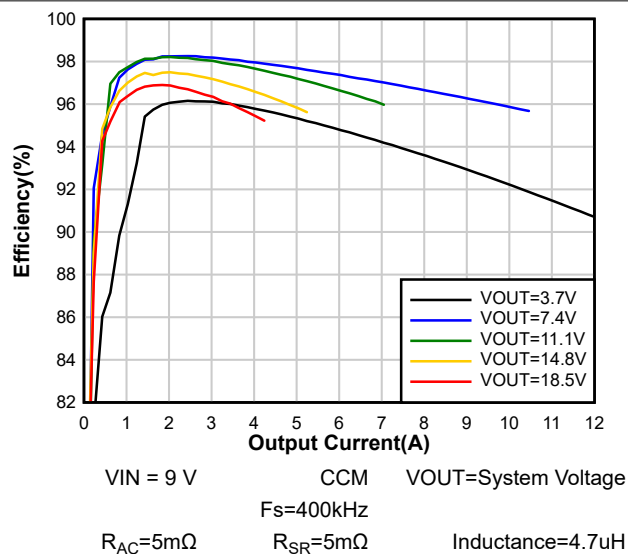
図 7-6. System Efficiency
