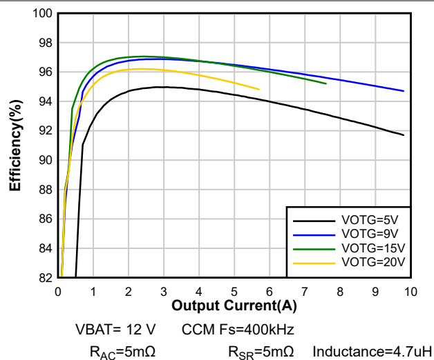
図 7-12. OTG Efficiency with 3S Battery
