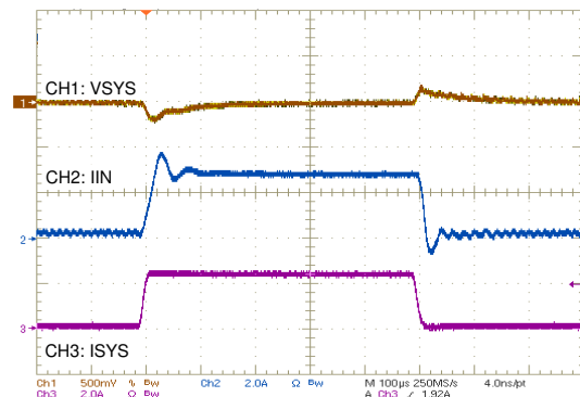
図 9-11. Switching During Buck Boost Mode
