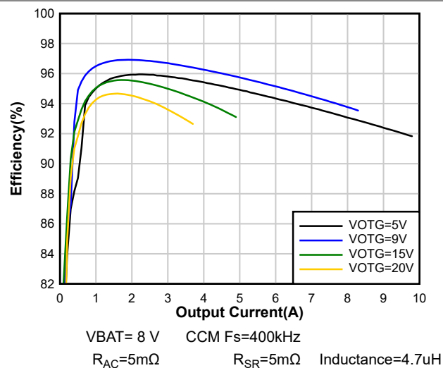
図 7-11. OTG Efficiency with 2S Battery
