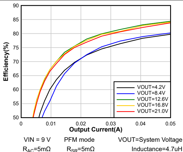
図 7-2. Light Load System Efficiency
