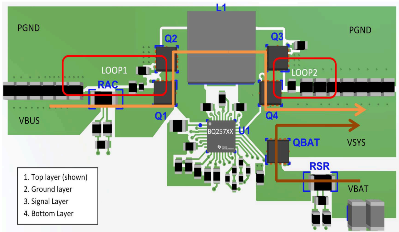
図 11-1. Buck-Boost Charger Layout Reference Example Top View
